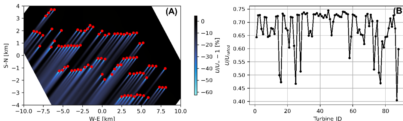
FIGURE 5 P2D-RANS simulation for a normalized wind speed of 0.73, wind direction of 50, and TI = 10\% . (A) Wind farm velocity field. (B) Rotor average wind speed for the various wind turbines.
