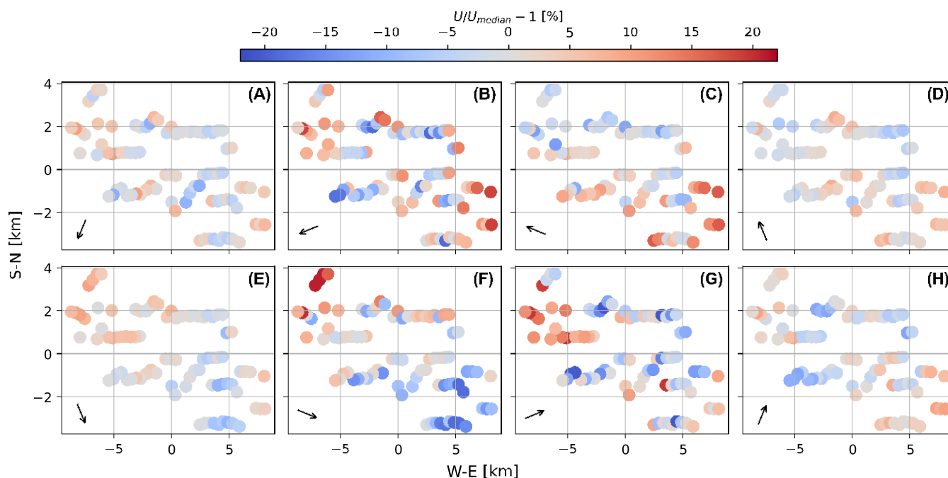
FIGURE 10 Average power for each turbine binning with reference wind speed between 7.5 and 8.5 m/s, reference TI between 7.5% and 12.5%, and reference wind direction between the following: (A) 0 and 45, (B) 45 and 90, (C) 90 and 135, (D) 135 and 180, (H) 180 and 225, (G) 225 and 270, (F) 270 and 315, (E) 315 and 360 (arrow pointing along bin center, wind moving from tail to tip).
