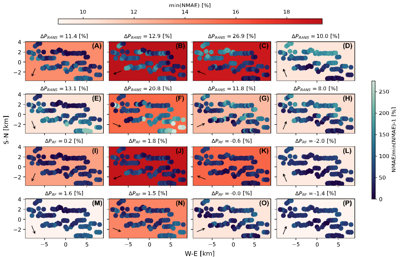
FIGURE 14 Bin NMAE of turbine power predictions for RANS (A–H) and RF (I–P) models, reference wind direction between the following: (A, I) 0 and 45, (B, J) 45 and 90, (C, K) 90 and 135, (D, L) 135 and 180, (H, M) 180 and 225, (G, N) 225 and 270, (F, O) 270 and 315, (E, P) 315 and 360 (arrow pointing along bin center, wind moving from tail to tip). The subplot color indicates the minimum NMAE for the subplot.
