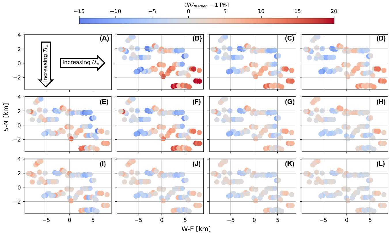
FIGURE 12 Percent deviation from median wind speed for SCADA data between reference wind directions of 157.5202.5. Reference wind speed is binned using the following intervals: [3 m/s, 5 m/s] (A, E, I), [5 m/s, 7 m/s] (B, F, J), [7 m/s, 9 m/s] (C, G, K), and [9 m/s, 11 m/s] (D, H, L). Reference TI is binned using the following intervals: [2.5%, 7.5%] (A–D), [7.5%, 12.5%] (E–H), and [12.5%, 17.5%] (I, J). All bins have SCADA data available except panel (A).
