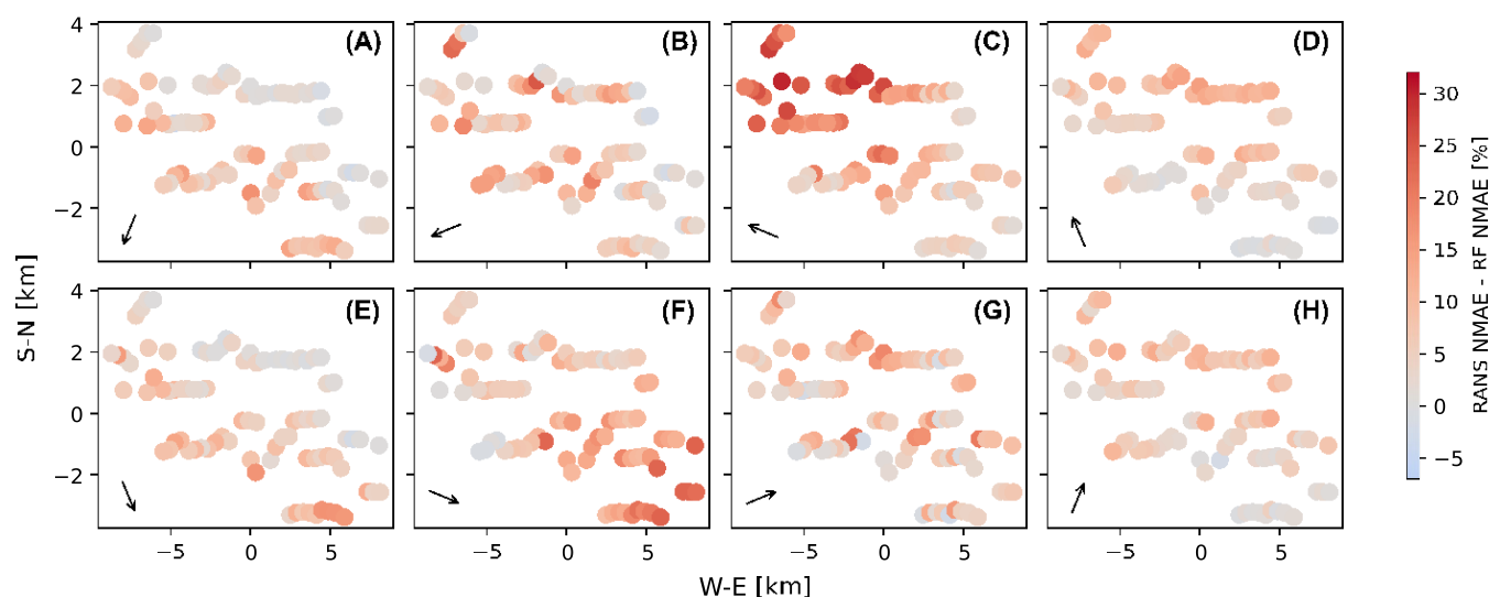
FIGURE 15 RANS bin NMAE for predicted turbine power minus RF bin NMAE, reference wind direction between the following: (A) 0 and 45, (B) 45 and 90, (C) 90 and 135, (D) 135 and 180, (H) 180 and 225, (G) 225 and 270, (F) 270 and 315, (E) 315 and 360 (arrow pointing along bin center, wind moving from tail to tip).
