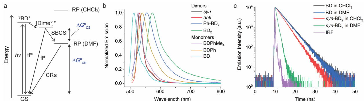
Figure 4. Overview of the photophysical pathways of the \beta -coupled dimers. (a) Photophysical diagrams of the dimers. The energy scale is arbitrary. Triplet excited states are not shown for brevity. (b) Emission spectra of the \beta -coupled BODIY dimers ( \lambda_{ex} = 540 nm for BD 2 and 490 nm for the rest). (c) Comparison of BD and syn -BD 2 emission lifetimes in chloroform and DMF ( \lambda_{ex} = 506 nm).
