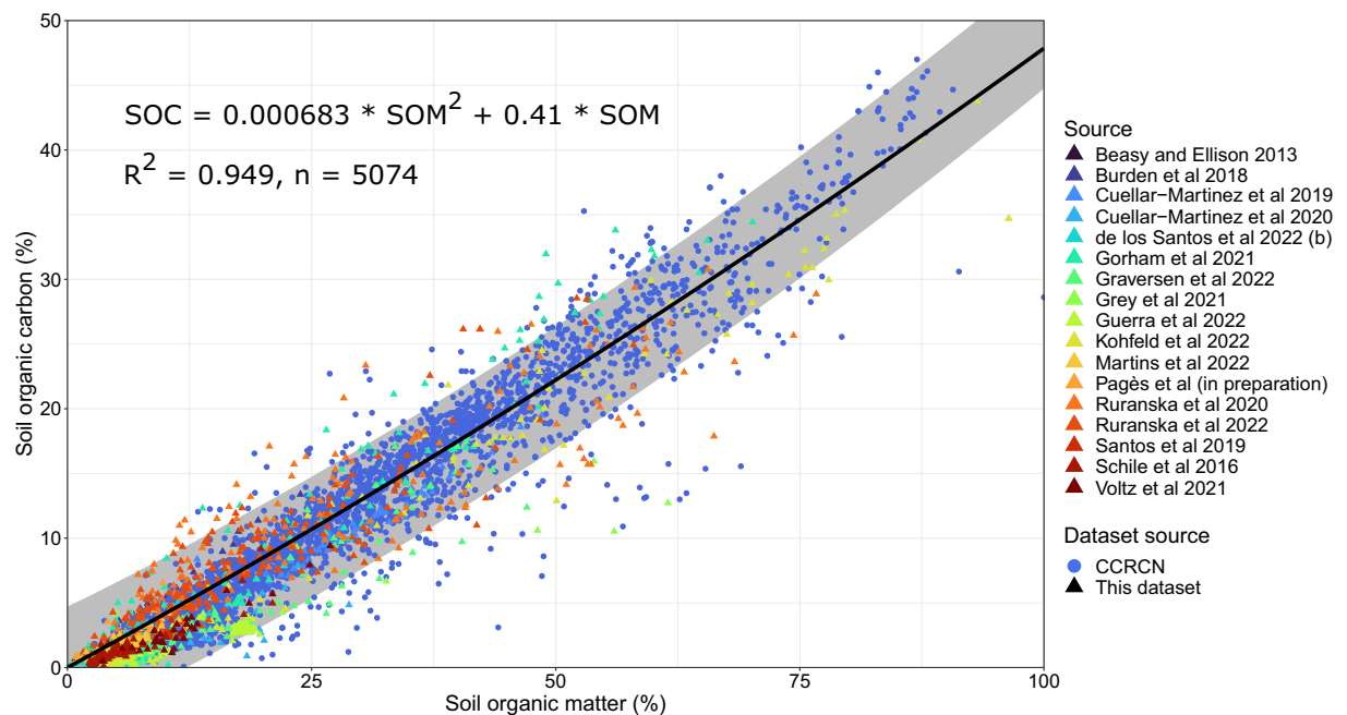
Fig. 4 Data points with both soil organic matter and soil organic carbon values, used to calculate the conversion equation for SOM to SOC (solid black line, with prediction intervals in grey). Data extracted from the Coastal Carbon Research Coordination Network (CCRCN) 19 are shown in circles, and values from this dataset are shown in triangles.
