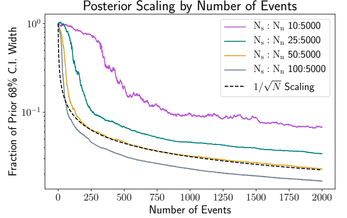
FIG. 12. Scaling with N_{\text{events}} of the ensemble R_{1.6} posterior 68% C.I. width as a fraction of the prior C.I. width for a 2000-event ensemble with R_{1.6} = 12.5 km and four different injected signal strengths. Note that the same behavior occurs for other C.I. percentages, but viewing the entire trend at low signal strengths for e.g. 95% C.I. requires many more events.
