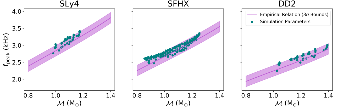
FIG. 8. Simulation parameters (post-merger peak frequency f_{\text{peak}} and chirp mass \mathcal{M} ) for each EoS, with the corresponding Vretinaris et al. [93] empirical relation with 3\sigma bounds for that EoS's value of R_{1.6} .
