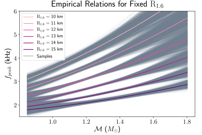
FIG. 2. Distribution of N_R = 1000 sampled relations, evaluated at a range of values of R_{1.6} , alongside our fitted empirical relations, likewise evaluated over the same range. The sampled distribution is consistent with the fit relation, and characterizes the relation's intrinsic uncertainty.
