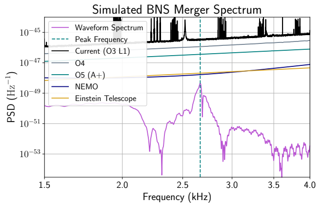
FIG. 1. GW power spectral density (PSD) of a simulated merger + post-merger waveform for the SFHX EoS (see §II F) with m_1 = 1.03 M_\odot and m_2 = 1.09 M_\odot , injected at a distance of 50 Mpc. The current, projected, and proposed detector noise PSDs discussed in this work are provided for reference: that of the LIGO Livingston detector during the 3rd LVK observing run (O3 L1); the projected LIGO sensitivities for the 4th and 5th LVK observing runs (O4 and O5), assuming LIGO A+ design sensitivity for O5 [61]; and the proposed NEMO and Einstein Telescope detectors (see § IV A) [62, 63]. The post-merger peak frequency of 2.67 kHz is marked.
