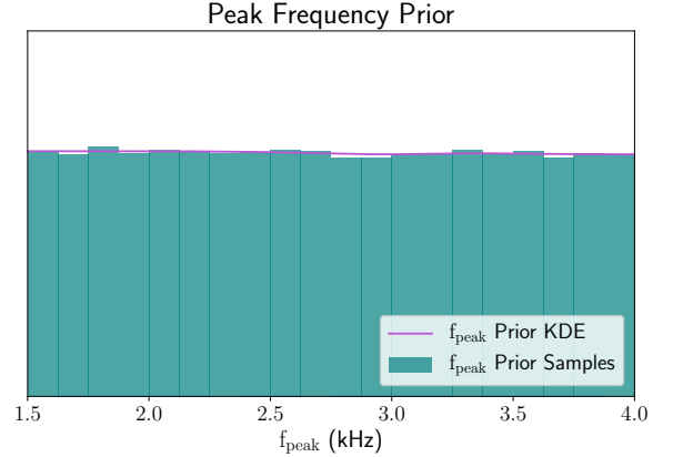
FIG. 6. Peak frequency prior samples, with a reflection-bounded KDE approximation of its probability distribution. These samples were computed from an ensemble of N=50 BayesWave analyses over simulated instrumental noise.
