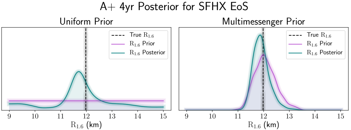
FIG. 15. R_{1.6} posteriors arising from a simulation of 4 years of operation at A+ sensitivity for the SFHX EoS, presented with both a uniform prior and the multimessenger prior of Huth et al. [35]. For the multimessenger (uniform) prior, we attain posterior means and 95% C.I. of R_{1.6} = 11.91^{+0.80}_{-0.56} km ( R_{1.6} = 11.9^{+2.6}_{-2.6} km). For reference, the multimessenger (uniform) prior means and 95% C.I. are R_{1.6} = 12.07^{+0.98}_{-0.77} km ( R_{1.6} = 12.0^{+2.9}_{-2.9} km). In the case of the multimessenger prior, we achieve a reduction in the 95% C.I. width of 0.39 km (22%).
