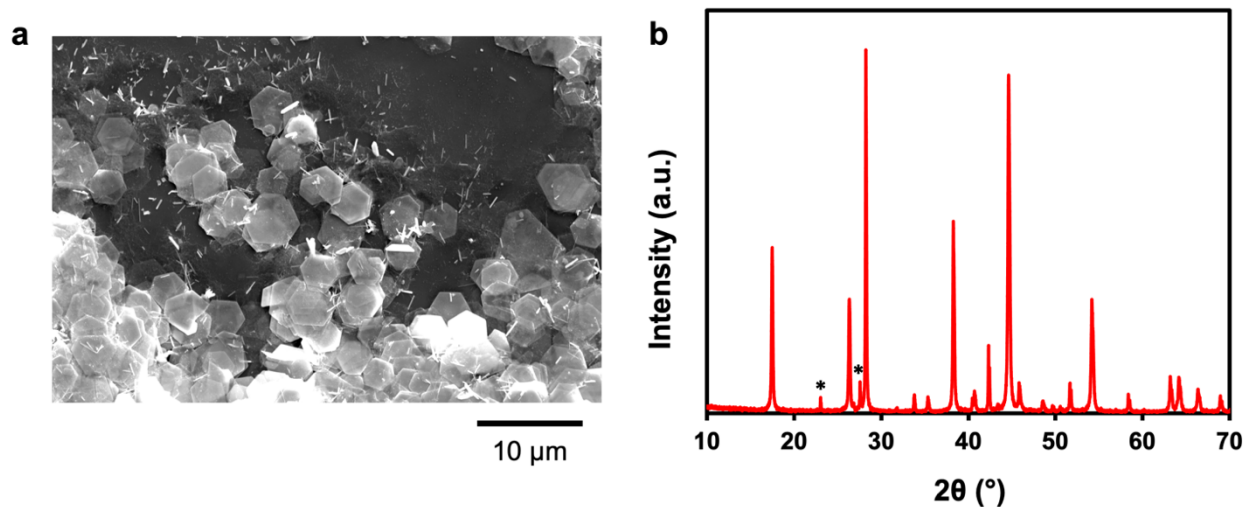
Figure S1. SEM micrograph (a) and PXRD pattern (b) of \text{Sb}_2\text{Te}_3 nanoplates with Te nanorod impurity. The asterisks in the PXRD pattern corresponds to elemental Te.
