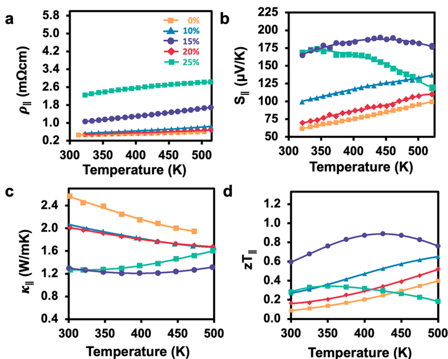
Figure 5. Thermoelectric properties in the parallel direction for nanoplate composites, showing (a) electrical resistivity, (b) Seebeck coefficient, (c) thermal conductivity, and (d) thermoelectric figure of merit, zT .
