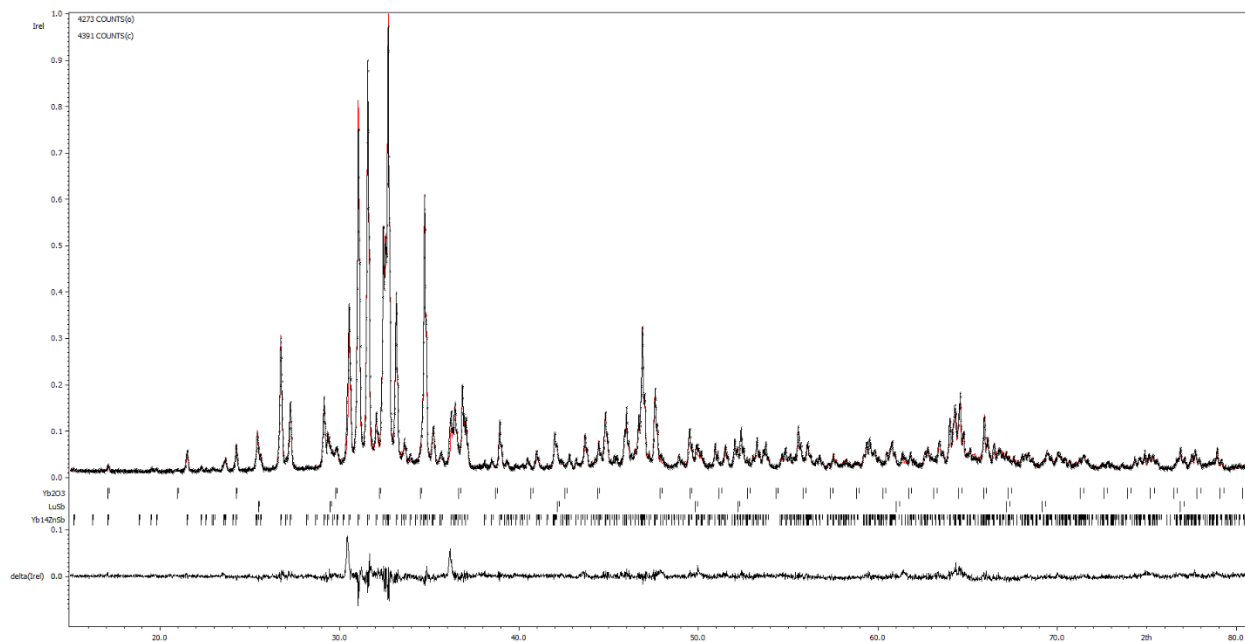
Figure S5: Rietveld refinement of the \text{Yb}_{14-x}\text{Lu}_x\text{ZnSb}_{11} x = 0.5 PXRD pattern.
