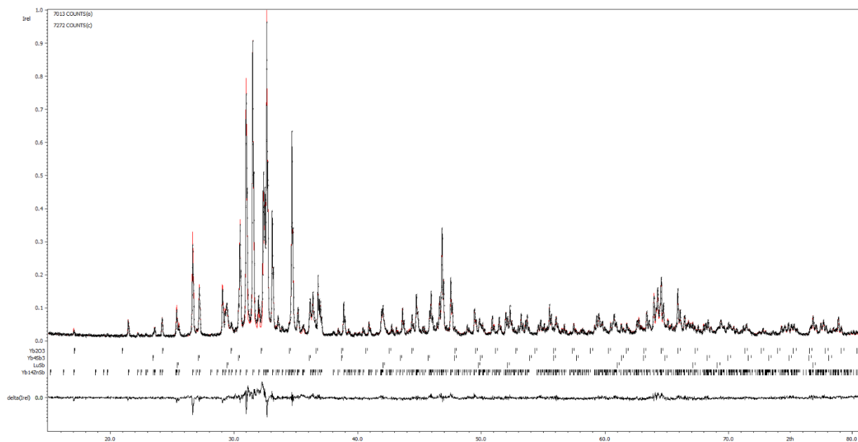
Figure S6: Rietveld refinement of the \text{Yb}_{14-x}\text{Lu}_x\text{ZnSb}_{11} x = 0.6 PXRD pattern.
