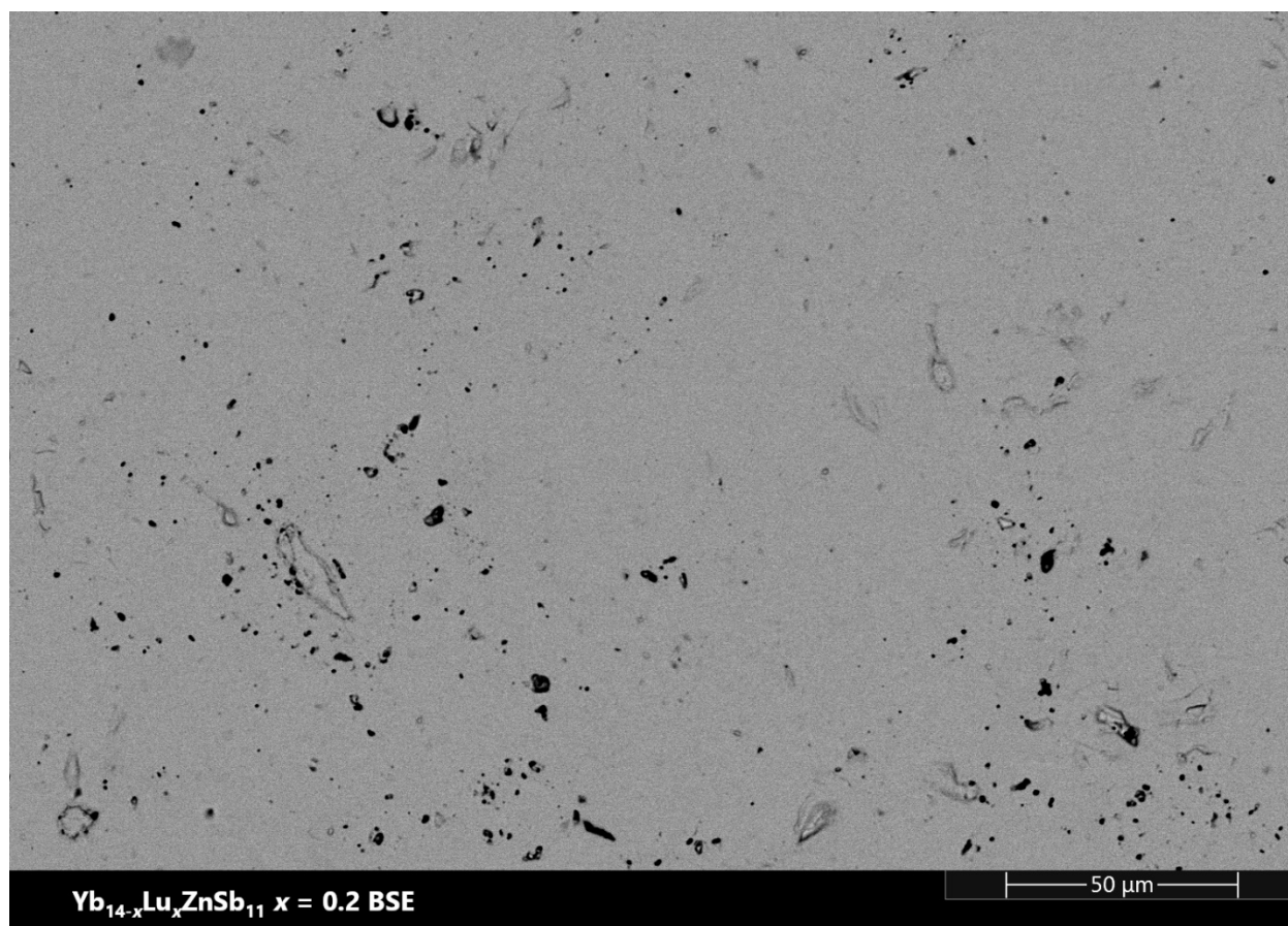
Figure S8. Backscattered electron micrograph of Yb 14-x Lu x ZnSb 11 , x = 0.2 .
