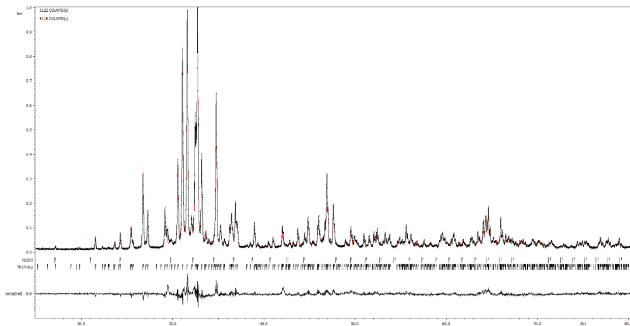
Figure S2: Rietveld refinement of the \text{Yb}_{14-x}\text{Lu}_x\text{ZnSb}_{11} x = 0.2 PXRD pattern.
