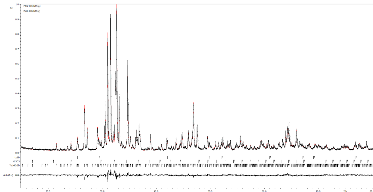
Figure S4: Rietveld refinement of the \text{Yb}_{14-x}\text{Lu}_x\text{ZnSb}_{11} x = 0.4 PXRD pattern.
