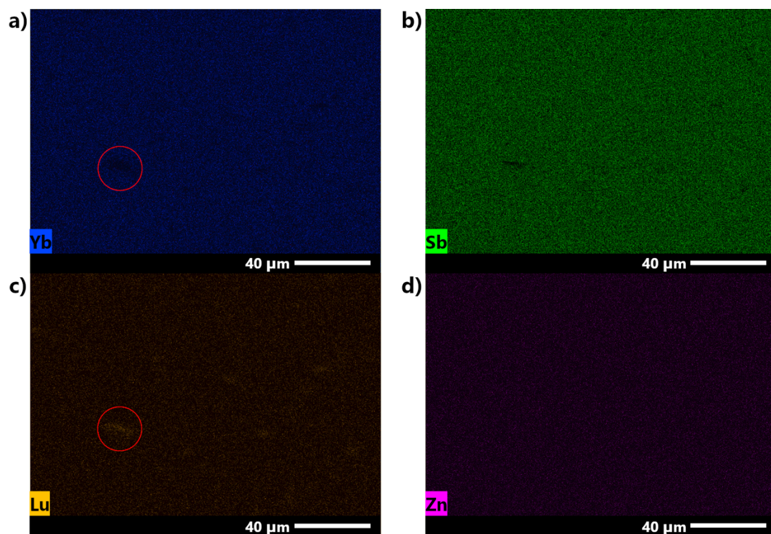
Figure S11. Elemental maps of a) Yb, b) Sb, c) Lu, and d) Zn from energy dispersive spectroscopy for \text{Yb}_{14-x}\text{Lu}_x\text{ZnSb}_{11} , x = 0.6 . Corresponding regions of deficient Yb and excess Lu are circled in red. The element is indicated in the bottom left with a 40 \mu\text{m} scale bar on the right.
