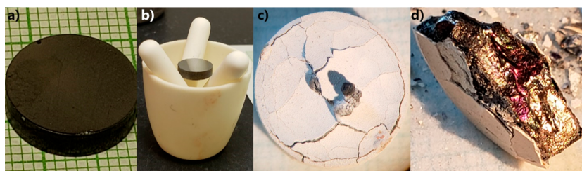
Figure 10. Pictures of the \text{Yb}_{14-x}\text{Lu}_x\text{ZnSb}_{11} ( x = 0.3 ) pellet (a,b) before and (c) after. (d) Cross-section of the pellet after oxidation.
