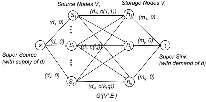
Fig. 2. DPP in BSN graph G(V, E) is equivalent to MCF problem in transformed flow network G'(V', E') . The first number in each parenthesis is the edge's capacity, and the second is its cost.
