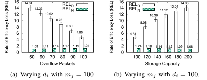
Fig. 4. Comparing Random and Greedy-N.
