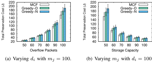
Fig. 8. Total preservation costs of different algorithms.
