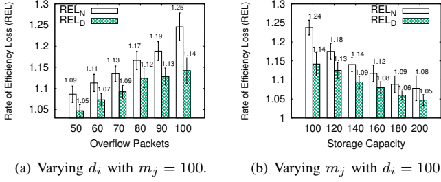
Fig. 5. Comparing Greedy-N and Greedy-D.
