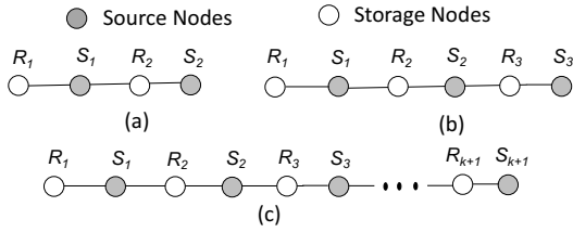
Fig. 3. Illustrating \text{PoA} = H(d) for NEs resulted from Algo. 1.
