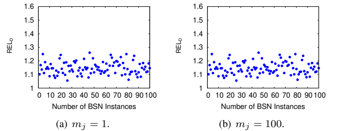
Fig. 7. Investigating the PoAs of Greedy-D.
