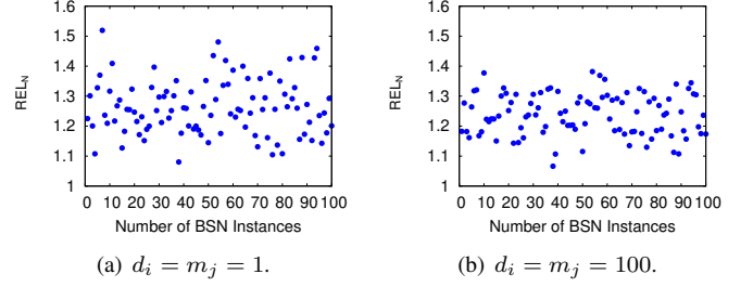
Fig. 6. Investigating the PoAs of Greedy-N.
