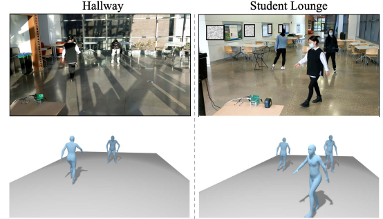
Figure 11: Cross-environment Experiments
