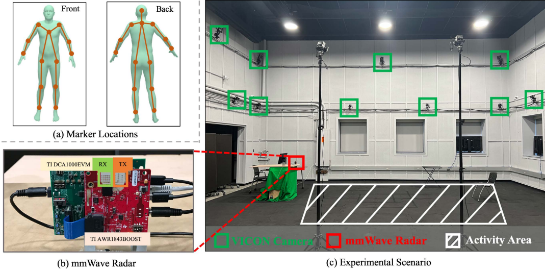
Figure 7: The Testbeds and the Experimental Scenario
