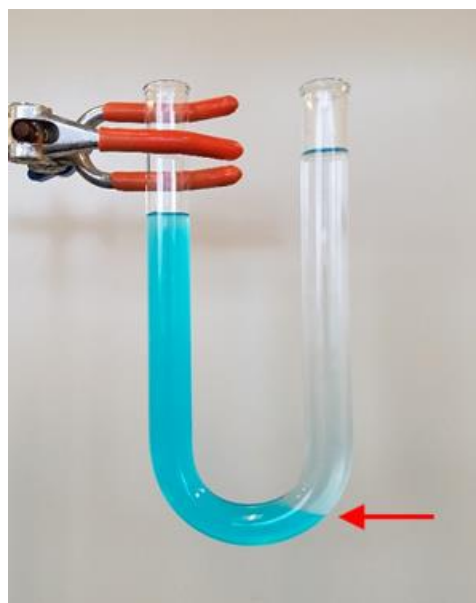
Figure 4: U-shaped manometer filled with two liquids of different densities. The arrow indicates the interface between the two liquids.
