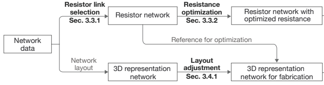
Fig. 3: A computational design pipeline for producing sensing network physicalizations. Rectangles represent output data or physical objects (see Sec. 3 for definitions). Arrows represent different processes. Processes that are bolded are new methods that we introduce (Sec. 3.3–Sec. 3.6).
