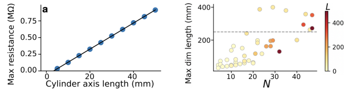
Fig. 7: Fabrication scalability analysis: (a) the maximum resistance we can create for different cylinder lengths; (b) the longest dimension lengths required for printing space, where 250 mm corresponds to the maximum printable size using a Prusa i3 MK3S+.
