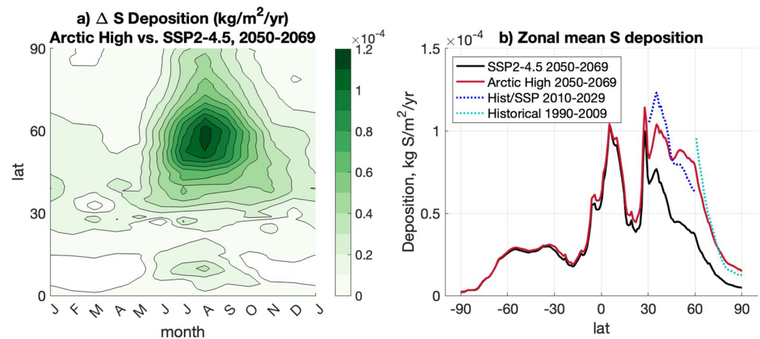
Figure 10. Changes to zonal mean sulfur deposition. Panel (a) displays the seasonal cycle of zonal mean sulfur deposition in kg/m²/yr for Arctic High 2050–2069 relative to SSP2-4.5 2050–2069. Panel (b) shows zonal mean sulfur deposition for Arctic High and SSP2-4.5, both averaged over 2050–2069; shading denotes standard error as described in Supporting Information S1 (Text S2). Included for comparison are mid-latitude and high-latitude sulfur deposition for Historical/SSP2-4.5 in the 2010–2029 and 1990–2009 periods, respectively, which are similar to the increased deposition under Arctic High; these are indicated by dotted lines. (Note: sulfur deposition data for Historical/SSP2-4.5 is taken from runs using the full-atmosphere (troposphere, stratosphere, mesosphere, lower thermosphere, or "TSMILT") configuration of WACCM (one ensemble member) instead of the MA configuration because deposition output was not saved for the MA simulations; emissions are the same for both configuration and tropospheric lifetime is short, so deposition should be similar).
