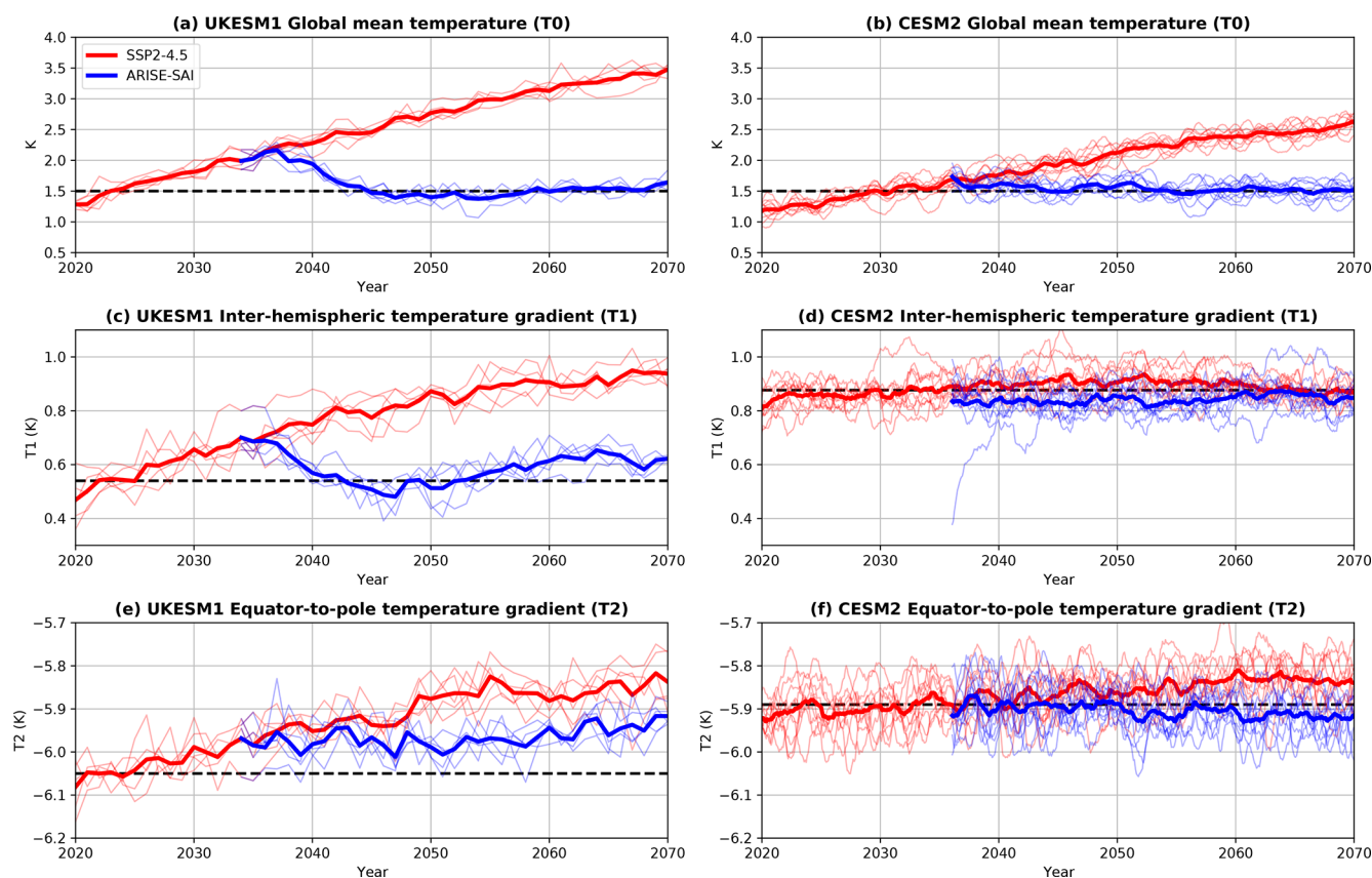
Figure 1. Comparison of global-mean temperature (T0), inter-hemispheric temperature difference (T1), and Equator-to-pole temperature gradient (T2) for the SSP2-4.5 simulations (red) and the ARISE-SAI-1.5 simulations (blue) for UKESM1 (a, c, e) and CESM2 (b, d, f). Thin lines represent individual ensemble members, whereas the thick lines show the ensemble mean. The temperature targets for the controller are shown by the dashed black lines.
