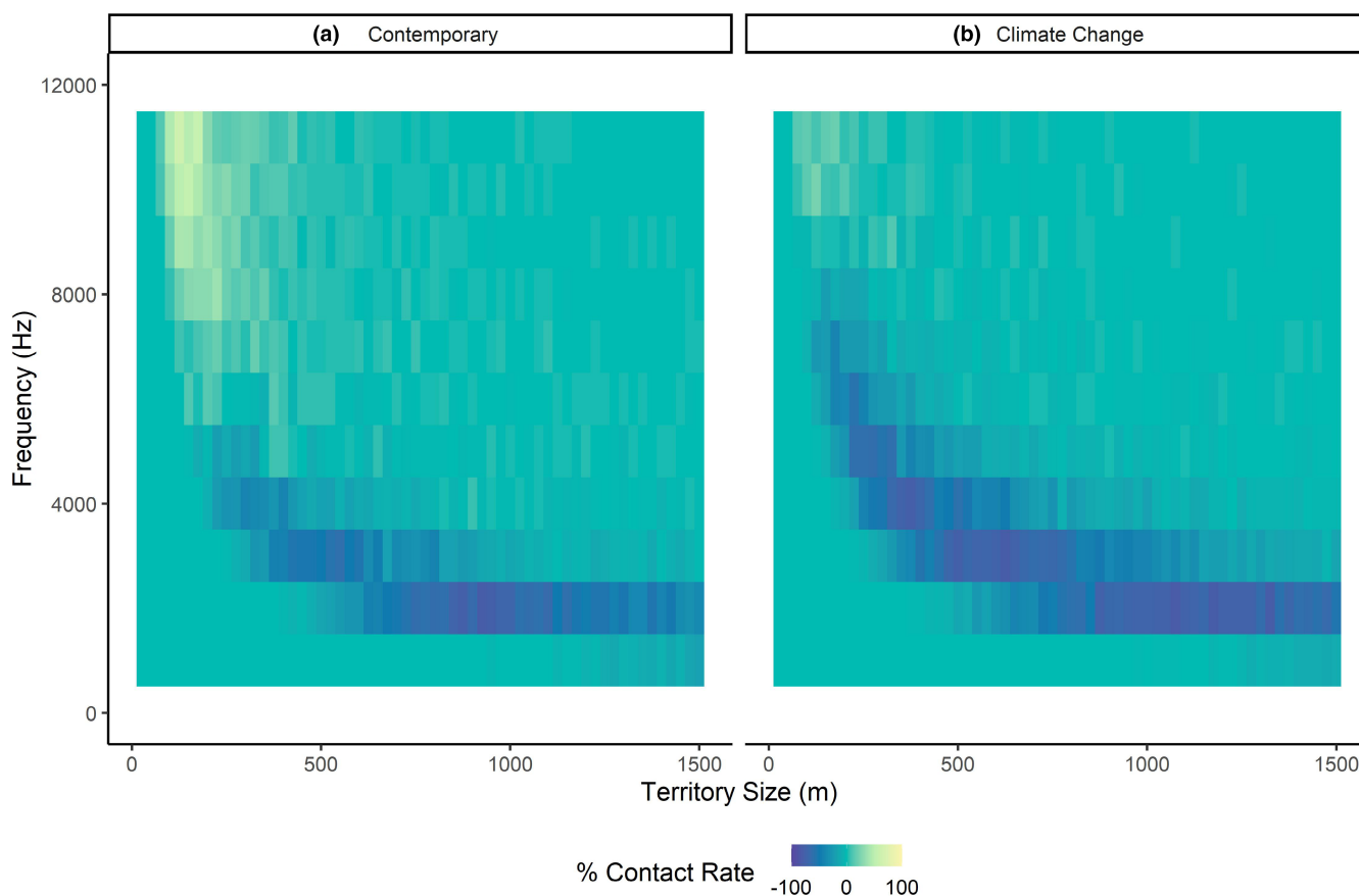
FIGURE 3 Heatmaps of frequencies affected by extreme temperatures across different territory sizes. We applied the ABM to multiple territory sizes ranging from 25m radius territories to 1500m radius territories across the audible bird song frequencies for the differences in drought versus contemporary weather data (a), and the differences in climate change drought versus climate change weather data (b). Cooler colors represent frequencies and territory sizes that would lead to fewer birds successfully contacting all neighbors under extreme conditions in both the extreme and climate change drought data, suggesting that selection may drive bird populations toward smaller territory sizes and higher frequency songs.
