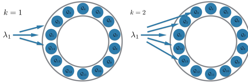
Fig. 1. k-nearest neighbor queue with k = 1 (left) and k = 2 (right).
