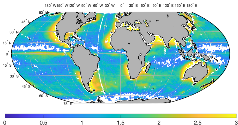
Figure 1. Geographic distribution of cutouts in our 98 % clear VIIRS dataset, shown using a \log_{10} -based scale of color intensity. Each equally sized (HEALPix) spatial cell, plotted as dots here, covers approximately 10\,000\text{ km}^2 . HEALPix cells with fewer than five VIIRS cutouts or fewer than five LLC4320 cutouts are shown in white. Land is shown as light gray. Meridional white line at \sim 35^\circ\text{ W} is due to an LLC4320 sampling artifact.
