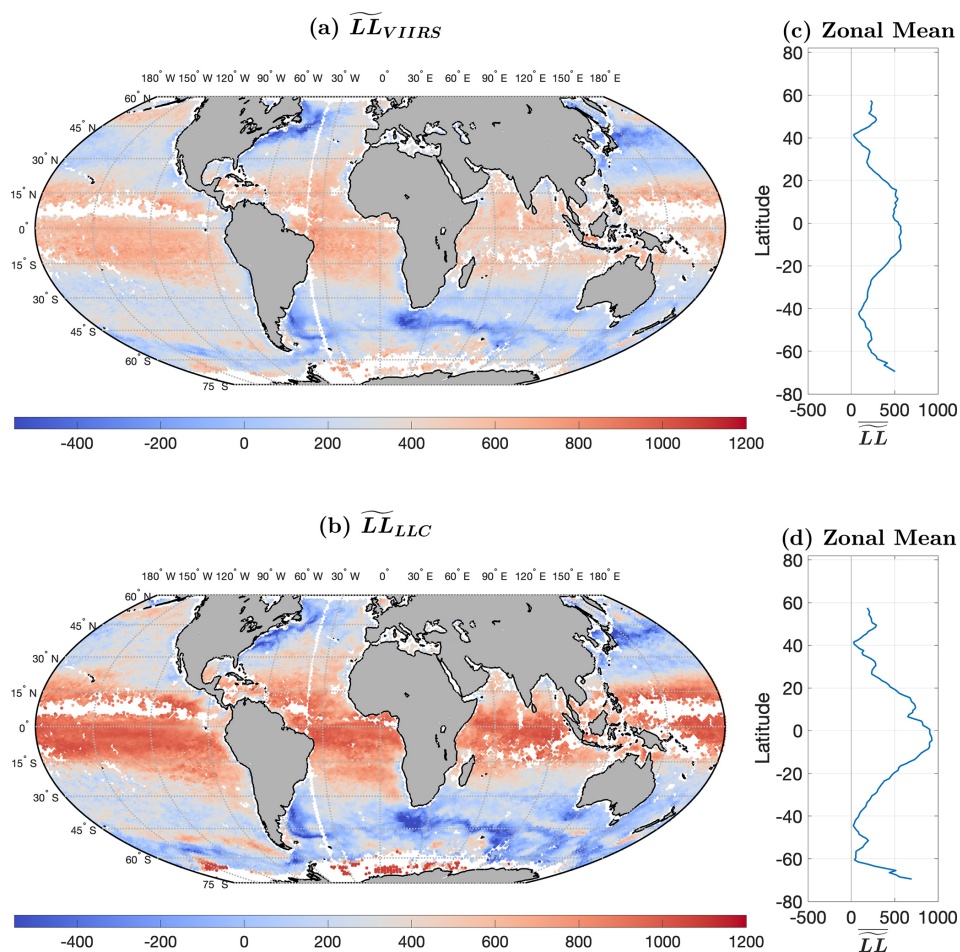
Figure 4. HEALPix median LL for (a) VIIRS cutouts ( \widetilde{LL}_{VIIRS} ), (b) \widetilde{LL}_{LLC} , (c) the zonal average of \widetilde{LL}_{VIIRS} , and (d) the zonal average of \widetilde{LL}_{LLC} . Each dot in (a) and (b) is associated with an equal-area HEALPix cell. White dots correspond to locations with fewer than five VIIRS cutouts and fewer than five LLC4320 cutouts in the HEALPix cell. Land is shown in gray.
