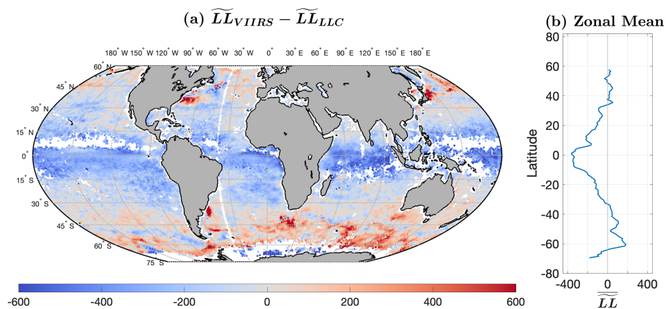
Figure 5. (a) \widetilde{LL}_{VIIRS} - \widetilde{LL}_{LLC} . (b) Zonal mean of \widetilde{LL}_{VIIRS} - \widetilde{LL}_{LLC} . It is apparent that the LLC4320 model has SST patterns with less structure in equatorial regions. In contrast, the dynamic regions of the global ocean (e.g., western boundary currents) exhibit lower \widetilde{LL}_{LLC} , indicating a higher degree of structure within these areas in the model output.
