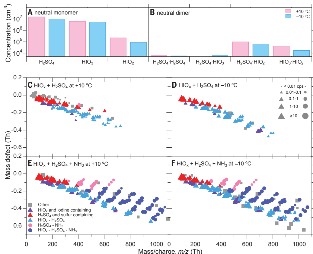
Fig. 3. Neutral and charged cluster composition during \text{HIO}_x\text{-H}_2\text{SO}_4\text{-NH}_3 nucleation. Background-subtracted neutral monomer (A) and dimer (B) concentrations in \text{HIO}_x\text{-H}_2\text{SO}_4 nucleation events at +10^\circ\text{C} (pink bars) and -10^\circ\text{C} (cyan bars).
