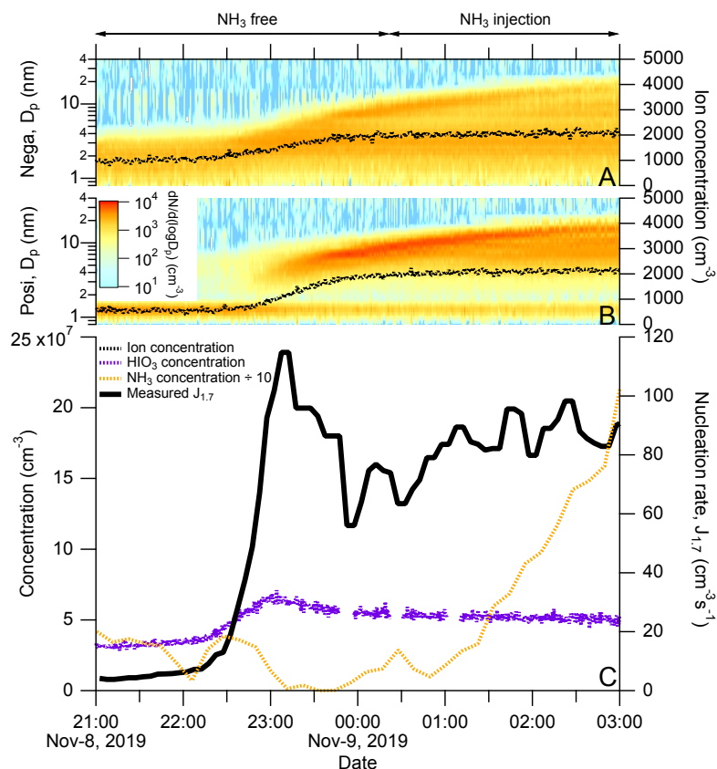
Fig. S8. Effect of \text{NH}_3 on \text{HIO}_x nucleation. (A) Negative ion size distribution, (B) positive ion size distribution and (C) vapor concentrations and nucleation rates. The results show that \text{NH}_3 has a negligible effect on \text{HIO}_x nucleation. Dashed lines represent total ion concentrations (dashed black), \text{HIO}_3 concentrations (dashed purple) and \text{NH}_3 concentrations (dashed yellow). The \text{NH}_3 concentrations are scaled down by a factor of 10 to optimize data presentation. The solid black line shows measured nucleation rates at 1.7 nm, J_{1.7} . The experimental conditions are 42.1 ppbv \text{O}_3 and 43.3 % RH. The results show that \text{NH}_3 up to 100 pptv does not significantly enhance iodine oxoacid nucleation.
