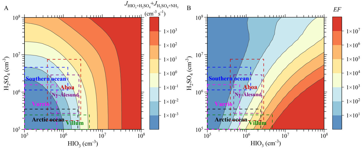
Fig. S10. Nucleation rate of \text{HIO}_x\text{-H}_2\text{SO}_4\text{(-NH}_3\text{)} and the enhancement by \text{HIO}_x at -10^\circ\text{C} . A) nucleation rate of \text{HIO}_x\text{-H}_2\text{SO}_4(+\text{NH}_3) estimated by summing up \text{HIO}_x\text{-H}_2\text{SO}_4 and \text{H}_2\text{SO}_4\text{-NH}_3 nucleation rates. The \text{NH}_3 concentration is assumed to be 10 pptv in pristine environments and the \text{HIO}_2 concentration is fitted from the experiments carried out at -10^\circ\text{C} (squares in Fig. S5). The condensation sink is assumed to be 0.0022 \text{ s}^{-1} in the calculations. The nucleation rate of \text{H}_2\text{SO}_4\text{-NH}_3 is calculated from our earlier studies(14). The 10 % and 90 % ranges from polar observations are drawn on top of the nucleation rates by dashed lines. B) Nucleation rate enhancement factor (EF), is calculated by dividing the nucleation rate from the sum of \text{HIO}_x\text{-H}_2\text{SO}_4 and \text{H}_2\text{SO}_4\text{-NH}_3 (10 pptv) nucleation rates to the \text{H}_2\text{SO}_4\text{-NH}_3 nucleation rate alone. The 10 and 90 percentiles from polar observations are drawn on top of the EF indicating that the nucleation rates might be significantly underestimated if not considering \text{HIO}_x . The results show \text{H}_2\text{SO}_4\text{-NH}_3 nucleation might be significantly enhanced by \text{HIO}_x under ambient conditions.
