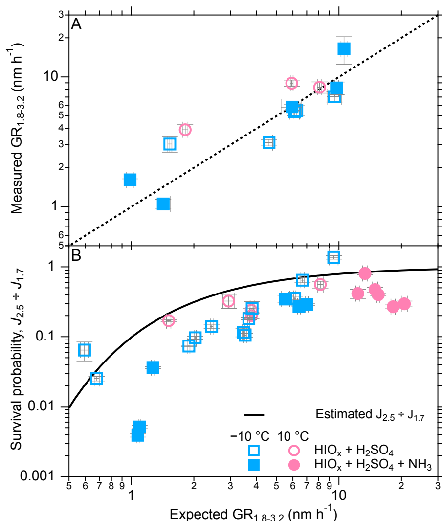
Fig. S9. Growth rate and survival probability. (A) measured growth rates between 1.8 to 3.2 nm by DMA-train versus the expected growth rates from kinetic \text{H}_2\text{SO}_4(33) and \text{HIO}_3(18) condensation at the concentrations corresponding to the measurement conditions. (B) survival probability of 1.7 nm particle growing to 2.5 nm, J_{2.5} / J_{1.7} . The J_{2.5} is measured with a condensation particle counter and the J_{1.7} is measured with a particle size magnifier. The estimated survival probability is calculated based on Lehtinen et al.(63, 64). Error bars show one standard deviation during the data selection period. Systematic errors resulting from uncertainties in the vapor concentrations (for estimating growth rates) and instrument cut-off sizes are not included in the plots. The results show that \text{HIO}_3 enhances \text{H}_2\text{SO}_4 stability in charged clusters under background \text{NH}_3 levels. At equal amounts of \text{HIO}_3 and \text{H}_2\text{SO}_4 , \text{NH}_3 does not further enhance the \text{H}_2\text{SO}_4 molar ratio. Additionally, \text{HIO}_3 contributes to charged cluster formation starting at dimers at -10\text{ }^\circ\text{C} and at tetramers at 10\text{ }^\circ\text{C} .
