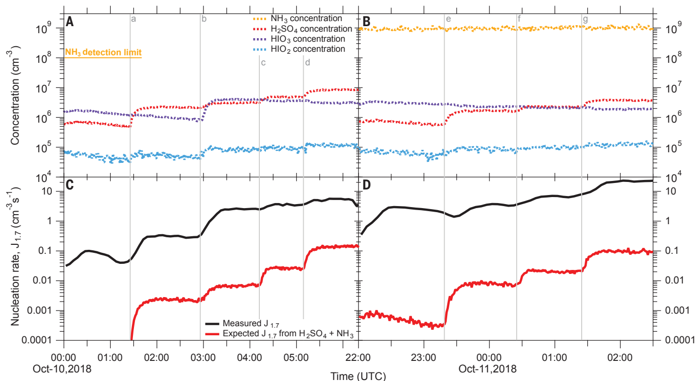
Fig. 1. New particle formation from HIO x -H 2 SO 4 and HIO x -H 2 SO 4 -NH 3 at -10°C.
