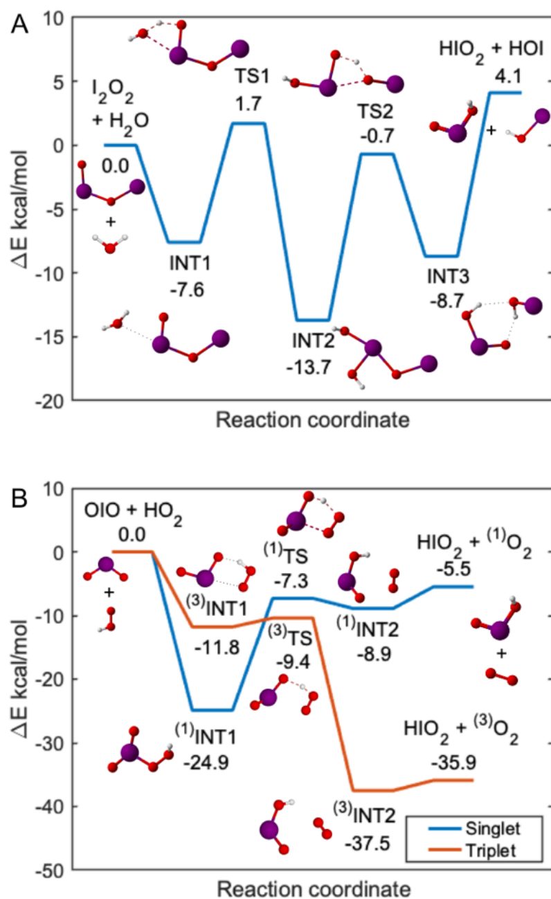
Fig. S4. Gas-phase formation mechanisms of HIO 2 . A) Stationary points along the potential energy surface of reaction \text{I}_2\text{O}_2 + \text{H}_2\text{O} \rightarrow \text{HIO}_2 + \text{HOI} and B) Stationary points along the potential energy surface of reaction \text{OIO} + \text{HO}_2 \rightarrow \text{HIO}_2 + {}^{(1,3)}\text{O}_2 . Zero-point corrected energies are shown on the y-axis and the reaction coordinate on the x-axis. Color coding: Purple – iodine, red – oxygen, white – hydrogen. Our results indicate that \text{I}_2\text{O}_2 + \text{H}_2\text{O} and \text{OIO} + \text{HO}_2 are potential reactions forming HIO 2 in the gas phase.
