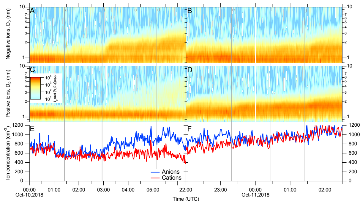
Fig. S1. Ion number size distribution from \text{HIO}_x\text{-H}_2\text{SO}_4 (A, C, E) and \text{HIO}_x\text{-H}_2\text{SO}_4\text{-NH}_3 (B, D, F) at -10^\circ\text{C} . (A, B) Negative ion number size distribution, (C, D) positive ion number size distribution and (E, F) ion concentrations. Ion-induced nucleation at background level of \text{NH}_3 levels only occurs at the negative channel (A) and the negative ion concentration is significantly higher than positive ions (E). However, ion-induced nucleation turns to bipolar (B, D) at ca. 40 pptv of \text{NH}_3 and the ion concentrations at both polarities are similar. The experimental conditions are the same as in Fig. 1: 41.1 ppbv \text{O}_3 , 63.5% RH, 2.3 ppbv \text{SO}_2 and 17.4 pptv \text{I}_2 (A, C, E), and 40.8 ppbv \text{O}_3 , 62.3% RH, 1.6 ppbv \text{SO}_2 and 67.2 pptv \text{I}_2 (B, D, F) with varying light intensities. Stages (a, c, d, e, f, g) enhanced the UVH light intensity (higher OH production rates) and stage (b) increased the green light intensity (higher \text{I}_2 photolysis rate). The results suggest that ion-induced \text{HIO}_x\text{-H}_2\text{SO}_4 nucleation proceeds in the negative channel, while ion-induced \text{HIO}_x\text{-H}_2\text{SO}_4\text{-NH}_3 nucleation proceeds in both the negative and positive channels.
