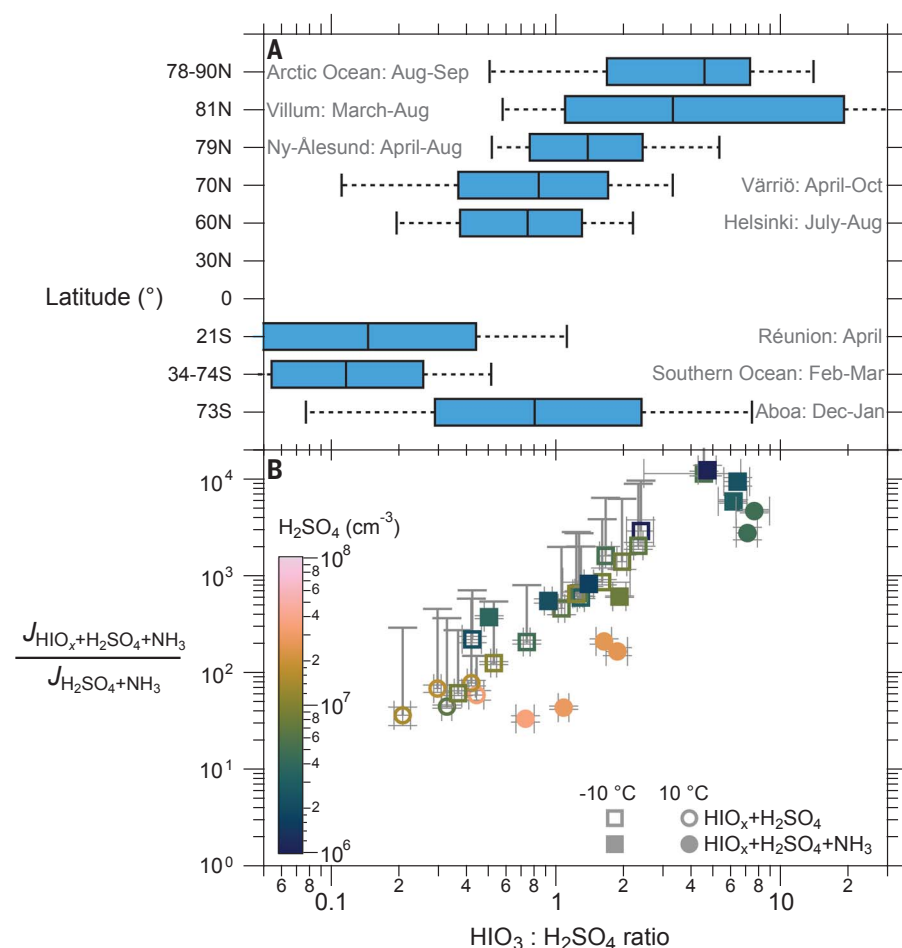
Fig. 4. \text{HIO}_x enhancement of \text{H}_2\text{SO}_4\text{-NH}_3 nucleation. (A) Box plot statistics of \text{HIO}_3:\text{H}_2\text{SO}_4 ratios measured around the globe, showing median values with 10 and 90% percentiles in the whiskers. The gray labels show the site name and months, with data covering >50% of the days. (B) Nucleation enhancement by \text{HIO}_x is calculated by dividing the measured J_{\text{HIO}_x+\text{H}_2\text{SO}_4+\text{NH}_3} to predict J_{\text{H}_2\text{SO}_4+\text{NH}_3} using CLOUD parameterizations (14). The median ratios at all sites are greater than 0.1, which infers at least a 10-fold nucleation rate enhancement by \text{HIO}_x . The enhancement is especially pronounced in polar regions where the \text{HIO}_3:\text{H}_2\text{SO}_4 ratio is consistently higher than 0.1. Thin symmetric error bars represent one standard deviation during the data selection periods. In the experiments without \text{NH}_3 injection (hollow markers), the \text{NH}_3 concentrations were below the instrument detection limit (4 pptv), which is adopted as a conservative estimate of J_{\text{H}_2\text{SO}_4+\text{NH}_3} . However, the actual \text{NH}_3 concentration is expected to be below 1 pptv, as all charged clusters are essentially \text{NH}_3 free (Fig. 3). The thick asymmetric error bars represent the systematic uncertainty assuming \text{NH}_3 equals 1 pptv. The \text{NH}_3 concentrations in experiments with \text{NH}_3 injection (filled markers) are well measured, and thus without asymmetric errors. The field observation sites are summarized in the methods.
