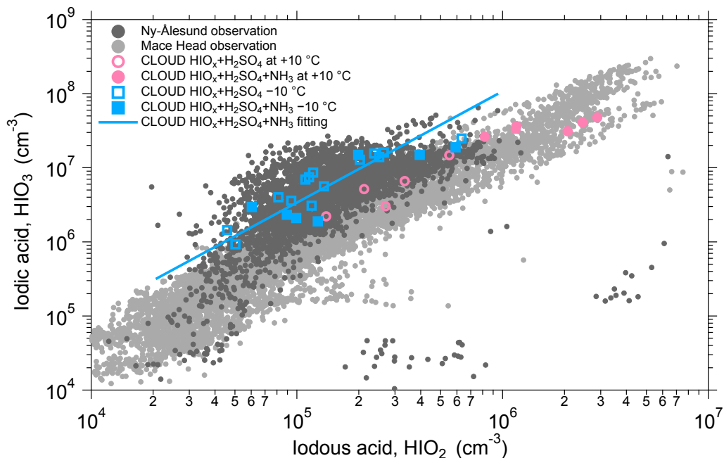
Fig. S5. \text{HIO}_3 vs \text{HIO}_2 in CLOUD and field observations. The Ny-Ålesund and Mace Head data sets are adopted from our earlier studies(17, 21). \text{HIO}_x\text{-H}_2\text{SO}_4\text{(-NH}_3\text{)} experiments are the same as the ones presented in Fig. 2. The solid blue line is a fitting to the CLOUD data at -10 °C with an expression of \log_{10}(\text{HIO}_2) = 0.6656 \times \log_{10}(\text{HIO}_3) + 0.6533 . The average temperature at Mace Head during September 2013 was around 14 °C and the temperature at Ny-Ålesund in March – August 2017 was between -19 and 10 °C. Our results show that both the ratio and absolute concentrations of \text{HIO}_2 and \text{HIO}_3 fall within the range measured at Mace Head and Ny-Ålesund.
