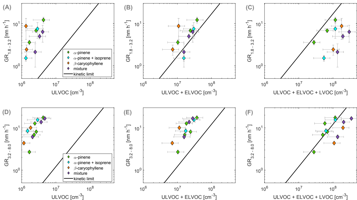
Figure S8 Particle growth rates as a function of vapour concentrations in different volatility classes. Particle growth rates during ozonolysis experiments for particle diameters between 1.8 and 3.2 nm as a function of (A) ULVOC, (B) ELVOC + ULVOC and (C) LVOC + ELVOC + ULVOC concentrations measured with NO 3 -CIMS and PTR3 and particle growth rates during ozonolysis experiments for particle diameters between 3.2 and 8 nm as a function of (D) ULVOC, (E) ELVOC + ULVOC and (F) LVOC + ELVOC + ULVOC. The black line shows the geometric limit of kinetic condensational growth (41).
