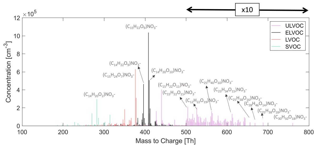
Figure S2 Chemical composition of \beta -caryophyllene oxidation products. Mass spectrum of \beta -caryophyllene oxidation products measured with \text{NO}_3 -CIMS. Here we show \beta -caryophyllene ozonolysis run #10. Concentrations of compounds exceeding 500 Th are multiplied by 10.
