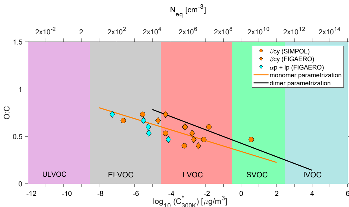
Figure S4 Volatility model at 300K used in this study. The volatility is calculated by the group-contribution method SIMPOL for \text{C}_{15}\text{H}_{22}\text{O}_x . We used the structures shown in Fig. S3 to know the functional groups to use SIMPOL ( \text{C}_{15} monomer and \text{C}_{15} dimer, in the BVOC mixture most of the \text{C}_{15} are from the cross dimer). This figure validates our parametrization that in the BVOC mixture \text{C}_{15} species are monomers. The parametrization can be used if up to \text{C}_{15} are monomers. The FIGAERO confirms that the molecules are closer to the monomer line. Species larger than \text{C}_{15} are dimers which include the peroxide groups.
