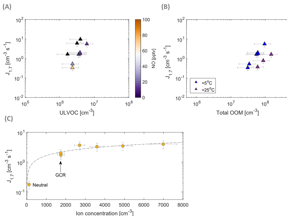
Figure S6 Effect of atmospheric conditions on particle formation rate. (A) Mixture runs ( \alpha -pinene+isoprene+ \beta -caryophyllene) at temperature = 5^\circ\text{C} and RH = 40%. Particle formation rate ( J_{1.7} ) as a function of ULVOC concentration, without NO are shown in black and coloured by NO concentration (colour bar). (B) Mixture runs ( \alpha -pinene+isoprene+ \beta -caryophyllene), RH = 40% and \sim 10 - 20 pptv NO, particle formation rate ( J_{1.7} ) as a function of OOM showing the temperature effect. (C) Mixture runs ( \alpha -pinene+isoprene+ \beta -caryophyllene), RH = 40% and \sim 10 - 20 pptv NO, particle formation rate ( J_{1.7} ) as a function of increasing ion concentration showing the importance of ions for pure biogenic nucleation. Neutral runs were achieved by turning on the high voltage field in the chamber, while increased ion concentration runs were performed using the adjustable \pi^+ beam from the CERN Proton Synchrotron, see Methods section.
