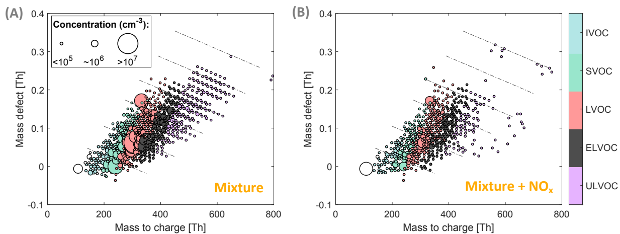
Figure S7 Chemical composition of BVOC oxidation results measured with NO 3 -CIMS in the absence and presence of NO x . Here we show example of (A) mixture runs \alpha -pinene+isoprene+ \beta -caryophyllene (run #14) and (B) \alpha -pinene+isoprene+ \beta -caryophyllene with ~30 pptv NO (run #22).
