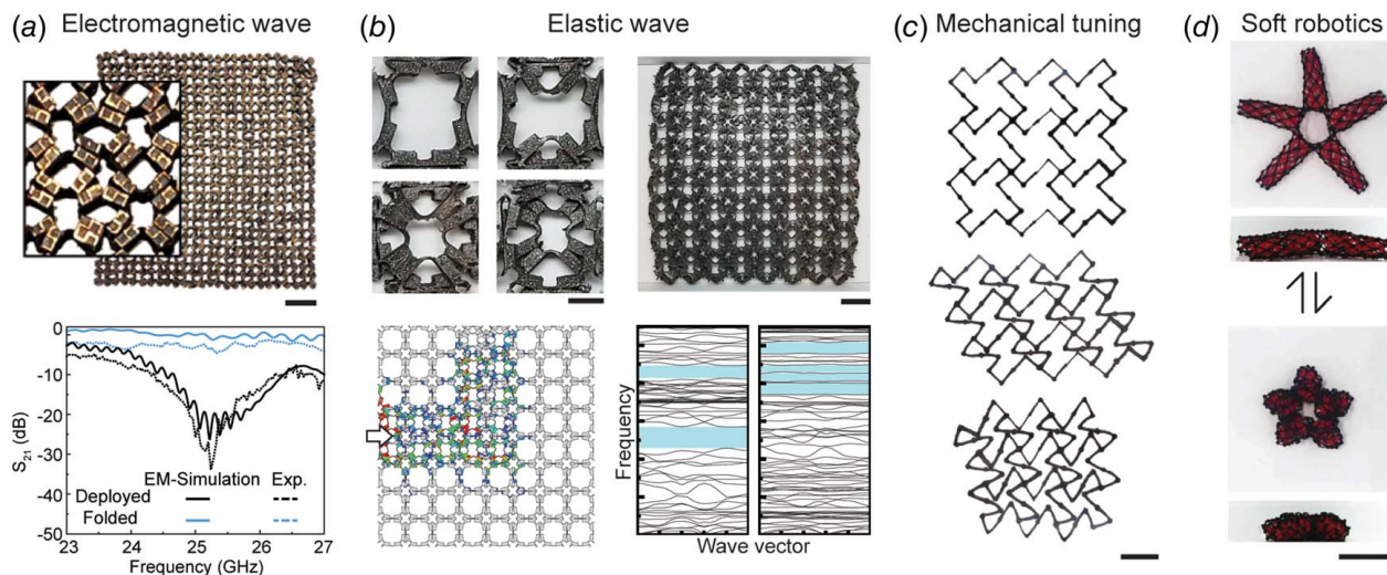
Fig. 2 Four examples of magneto-mechanical metamaterials. (a) Magneto-mechanical metamaterial utilized as a conformal electromagnetic wave filter. (Reproduced from Wu et al. [7] with permission from Wiley-VCH GmbH). Scale bar: 20 mm. (b) Area-preserving bilayer magneto-mechanical metamaterial with applications in elastic wave control and waveguide. Scale bars left to right: 5 mm and 20 mm. (Reproduced from Sim et al. [1] with permission from Wiley-VCH GmbH). (c) 3D printed magneto-mechanical metamaterial with the ability to demonstrate either positive or negative Poisson's ratio. (Reproduced from Ma et al. [15] with permission from American Chemical Society). Scale bar: 10 mm. (d) Tensegrity-based magneto-mechanical metamaterial with applications in soft robotics. (Reproduced from Lee et al. [19] with permission from the American Association for the Advancement of Science). Scale bar: 50 mm.
