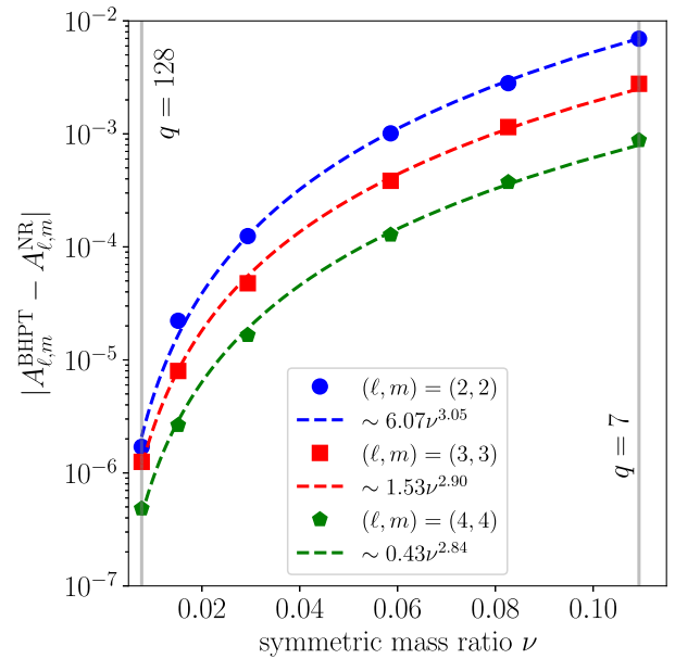
FIG. 6. We show the amplitude differences \delta A_{\ell,m} between ppBHPT and NR data at the merger (denoted by the maximum amplitude in the (2, 2) mode) for (2, 2) (blue circles), (3, 3) (red squares) and (4, 4) (green pentagons) modes for mass ratios q = [7, 15, 32, 64, 128] . Additionally, we show the best-fit functions for each mode in terms of \nu . More details are in Sec. IV A.
