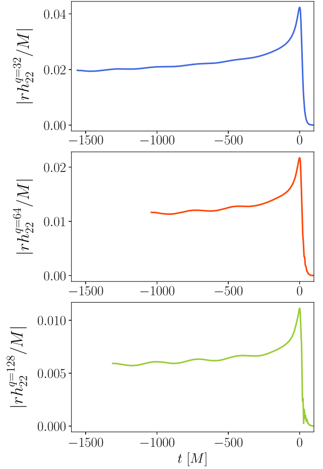
FIG. 10. We show the amplitudes of the (2,2) mode in RIT-NR waveform data for three different mass ratios: q = [32, 64, 128] . In all cases, we see modulations in the amplitudes due to residual eccentricity. More details are in the Appendix.
