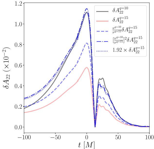
FIG. 5. We show the amplitude difference \delta A_{22} between ppBHPT and NR for q = 10 (solid gray line) and q = 15 (solid red line). Furthermore, we show the amplitude difference for q = 15 after rescaling them with different powers of the ratio of symmetric mass ratios (blue lines). More details are in Sec. IV A.
