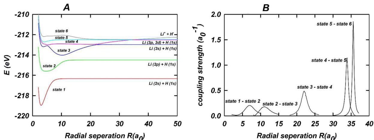
FIG. 7. (a) PECs of Li – H using AVQZ-ET2 basis set in MOLPRO. (b) NACMEs of Li – H using AVQZ-ET2 basis set in MOLPRO.
