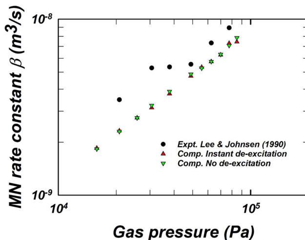
FIG. 11. Xe – F MN rate constant \beta(p_g) \sigma(v) . Experimental data (“Expt.”) reported by Lee and Johnsen 61 are plotted along with LD trajectory simulation calculations (“Comp.”) of the current study for Xe – F ^2\Pi^+ states.
