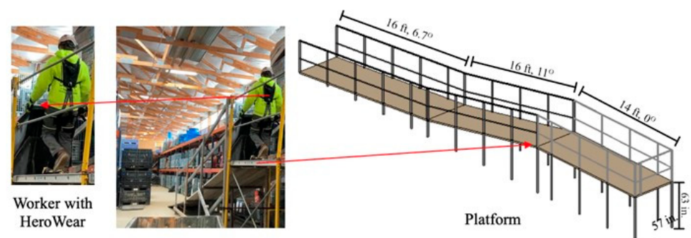
Figure 2. Pushing/emptying a construction gondola on a platform.
