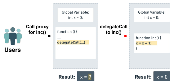
Figure 3: delegatecall Instruction
