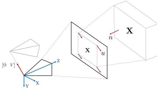
Fig. 3: By the pinhole model, a scene point \mathbf{X} is projected to image point \mathbf{x} . The camera “perceives” movement of \mathbf{x} as optical flow \mathbf{u} .
