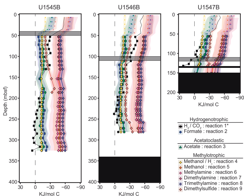
Fig. 2 Gibbs energies, \Delta G_r , of the nine methanogenic catabolic pathways considered in this study as a function of sediment depth at the three study sites. The solid lines represent average \Delta G_r values and the shaded envelopes around them refer to the possible range of \Delta G_r for that reaction based on a range of substrate concentrations (see Supplementary Table 2). The dashed lines above 50 mbsf indicate methane concentrations were below the detection limit and an activity of 10^{-7} was used in the calculations. The vertical dashed black lines refer to \Delta G_r = 0 . The black blocks indicate a magmatic sill, and the grey blocks represent the sulfate-methane transition zone, SMTZ, at each site. *No ranges for the Gibbs energies of hydrogenotrophic methanogenesis are shown because in situ measurements of \text{CO}_2 and \text{H}_2 were used rather than a range of substrate concentrations (see methods).
