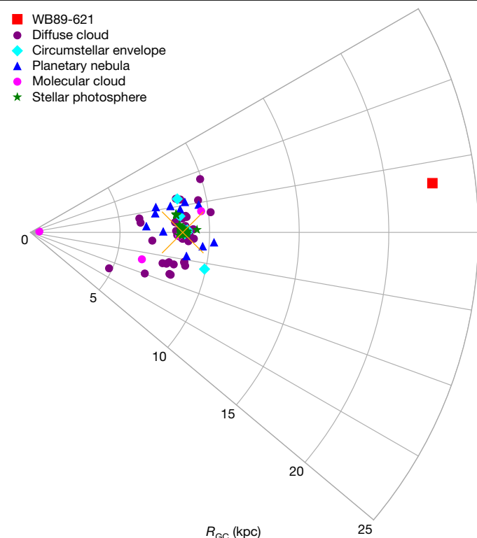
Fig. 1 | Currently known Galactic distribution of phosphorus. A graphic illustrating the Galactic distribution of phosphorus in the range 0–25 kpc from the Galactic Centre, as identified from stellar and interstellar observations. Detections by atomic transitions in stellar photospheres are denoted by green stars (from ref. 2 and references therein), in diffuse clouds by purple circles (ref. 16 and those therein 17–19 ), and in planetary nebulae by blue triangles 6–15 , while magenta circles and cyan diamonds mark the identifications in molecular clouds and circumstellar envelopes from molecular lines 25,34–36,40 . The red square shows the position of WB89-621. The orange X indicates the solar system. The APOGEE survey detections are not shown per possible contamination. WB89-621 is the only known source of phosphorus in any form beyond 12 kpc.
