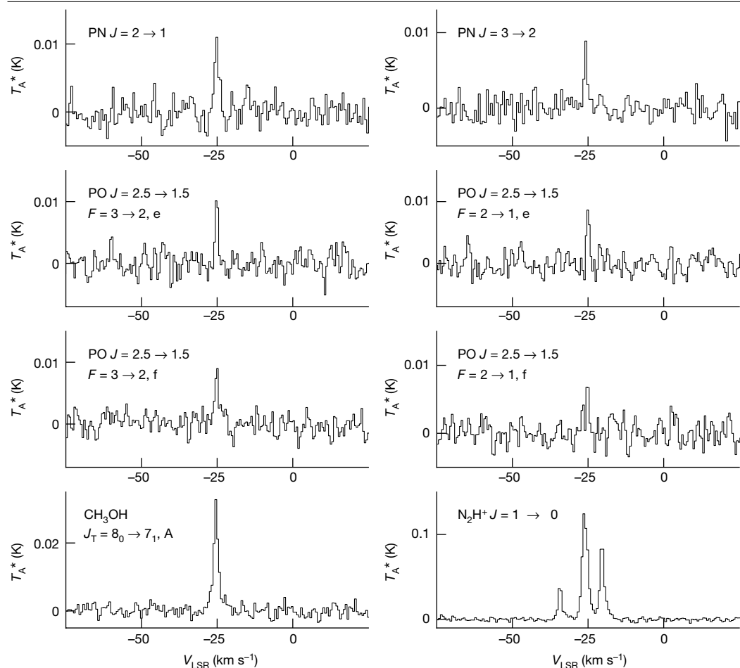
Fig. 2 | Spectra of molecular rotational transitions of PO, PN and other species in molecular cloud WB89-621. Spectra are plotted as intensity ( T_A^* ), in mK, versus V_{\text{LSR}} , in kilometres per second. The top two panels show the J = 2 \rightarrow 1 and J = 3 \rightarrow 2 transitions of PN, followed by the four hyperfine/lambda-doubling components of the J = 2.5 \rightarrow 1.5 transition of PO. The bottom two panels display the \text{N}_2\text{H}^+ J = 1 \rightarrow 0 and \text{CH}_3\text{OH } J_T = 8_0 \rightarrow 7_1, A transitions. Each panel includes the molecular species and quantum numbers corresponding to the rotational transition shown. The J = 2 \rightarrow 1 line of PN (156 kHz spectral resolution) was measured with the 12 m antenna of the ARO, while all others were observed using the IRAM 30 m telescope (200 kHz spectral resolution).
