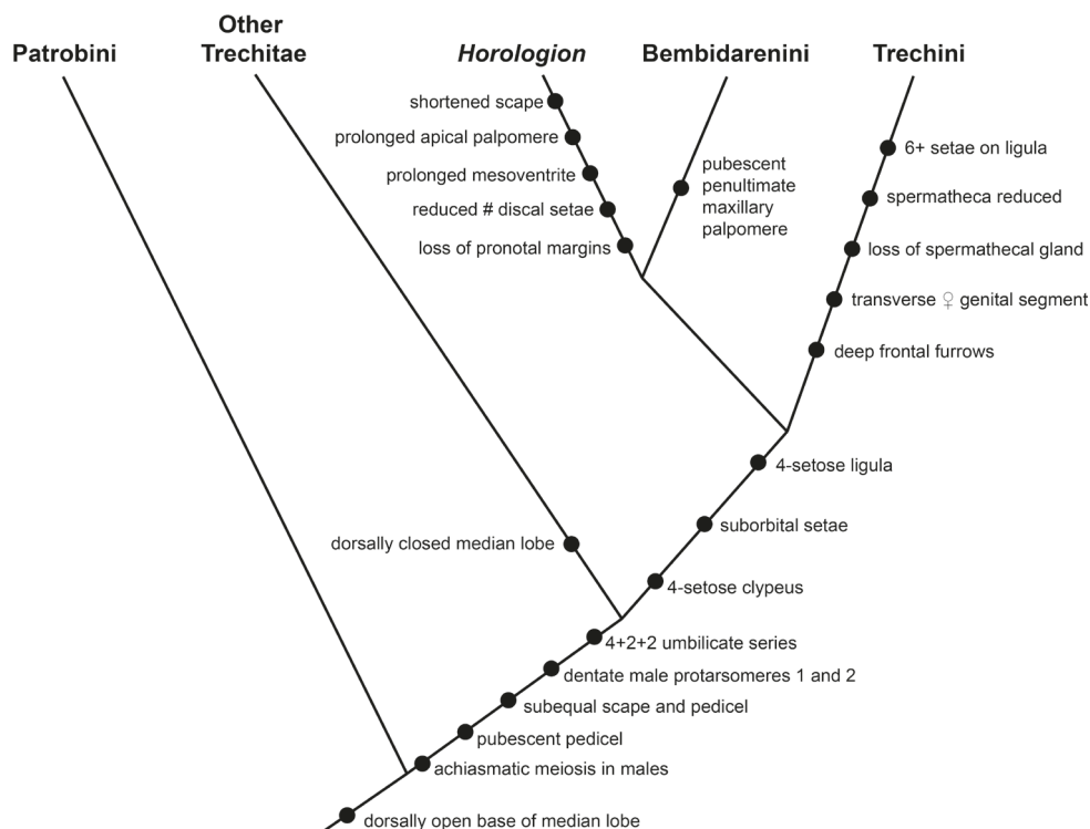
Figure 14. Phylogenetic tree of a portion of Trechinae showing proposed synapomorphies of clades. Topology is that of Fig. 4.
