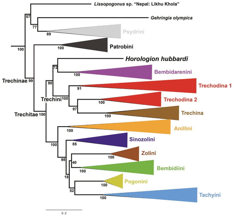
Figure 4. Summary of the maximum likelihood tree of Trechinae from IQ-TREE analysis of 8-gene concatenated matrix. Standard bootstrap support values are shown below nodes. For complete phylogenetic tree showing details within each clade, see Suppl. material 4.
