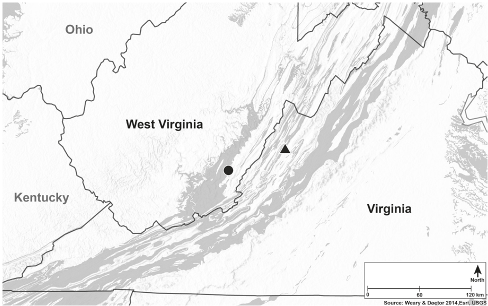
Figure 13. Distribution map of species of Horologion . Black triangle: Horologion hubbardi , black circle: Horologion speokoites . Grey shaded areas represent exposed karst (Weary and Doctor 2014).
