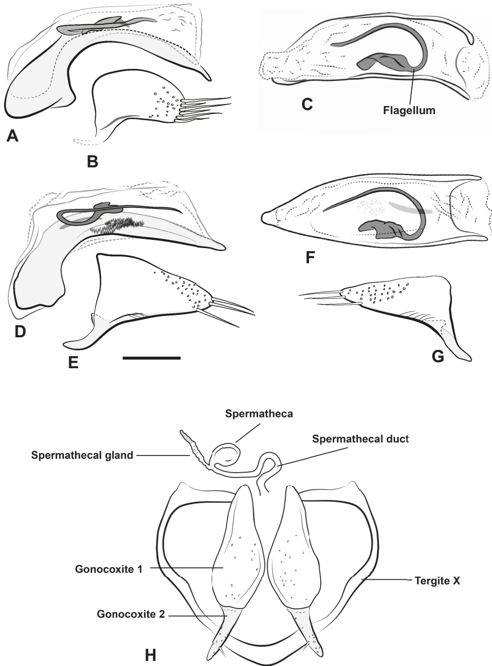
Figure 9. Genitalia of Horologion species A H. speokoites median lobe, left lateral aspect B H. speokoites left paramere, left lateral aspect C H. speokoites median lobe, dorsal aspect D H. hubbardi median lobe, left lateral aspect E H. hubbardi left paramere, left lateral aspect F H. hubbardi median lobe, dorsal aspect G H. hubbardi right paramere, right lateral aspect H H. hubbardi female genitalia, ventral aspect A–C after Valentine (1932). Scale bar: 0.1 mm.
