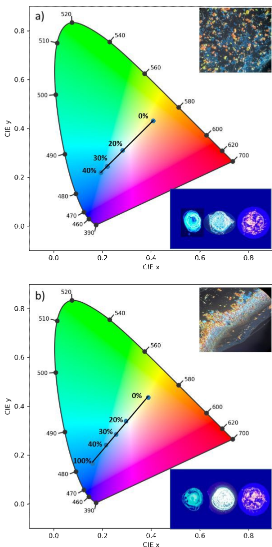
Figure 10. CIE plot establishing color-tuning capabilities of symmetrically substituted TTz-based dialkoxypheyl crystals. a) (MeOPh) 2 TTz crystals were mixed with (PrOPh) 2 TTz crystals at varying weight %. b) Crushed (MeOPh) 2 TTz crystals were mixed with (BuOPh) 2 TTz crystals at varying weight %. Selective weight proportions are plotted for clarity. Top Inset: Optical microscopic image of crystalline admixtures at 4:1 wt% of the symmetrically substituted TTzs illuminated by 400 nm lamp and viewed at 10x. Bottom Inset: Photographs of (PrOPh) 2 TTz/(BuOPh) 2 TTz (left); (MeOPh) 2 TTz (right); and multi-TTz crystalline white-light emissive blend illuminated by 400 nm lamp.
