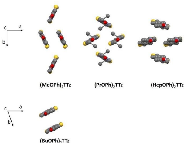
Figure 2. Crystal packing diagram of (C_nOPh)_2TTz unit cell. Top panel: Herringbone packing mode series; Bottom panel: slipped stack packing mode. H atoms are omitted for clarity.
