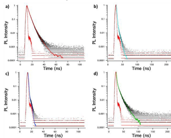
Figure 8. Singlet emission lifetime decay of a) (MeOPh) 2 TTz, b) (PrOPh) 2 TTz, c) (BuOPh) 2 TTz, d) (HepOPh) 2 TTz crystals.
