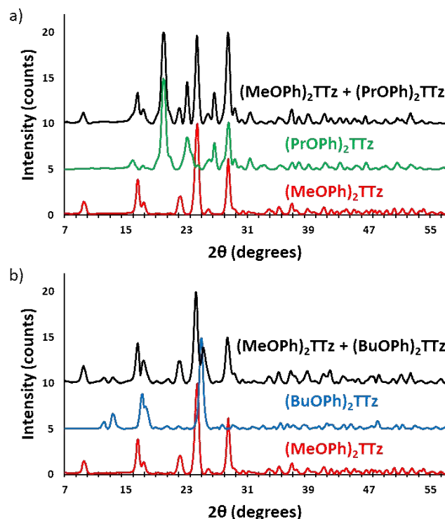
Figure 9. Powder X-ray diffractograms of parent TTz crystals and their blends. a) Set 1: (MeOPh) 2 TTz, (PrOPh) 2 TTz, and (MeOPh) 2 TTz + (PrOPh) 2 TTz crystalline blend; b) Set 2: (MeOPh) 2 TTz, (BuOPh) 2 TTz, and (MeOPh) 2 TTz + (BuOPh) 2 TTz crystalline blend.
