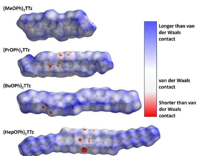
Figure 4. Normalized d_{\text{norm}} mapping images of the Hirshfeld surface analysis of the TTz crystals.
