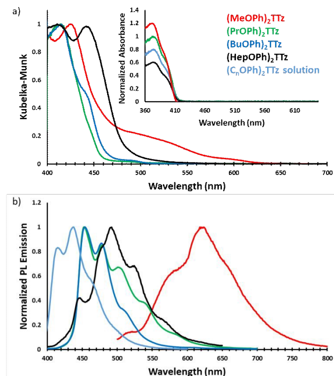
Figure 5. Steady state photophysical characteristics of symmetrically substituted dialkoxyphenyl TTz crystals. a) Absorption spectra of TTz crystals obtained via diffuse reflectance spectroscopy. Inset: UV-Vis absorption spectra of TTzs in solution state. b) Photoluminescence spectra of TTz crystals and solution.
