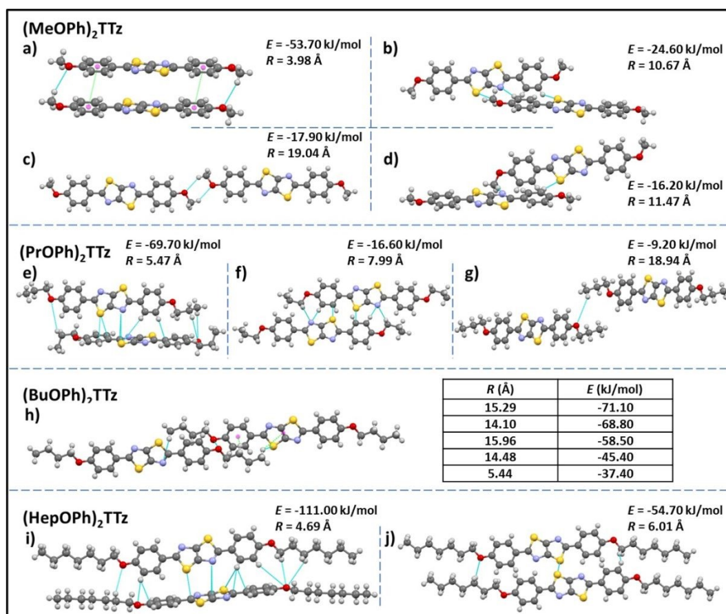
Figure 3. Unique intermolecular non-covalent interactions and orientation among (C_nOPh)_2TTz extrapolated from crystal packing and modeling studies. E is the total energy of interaction among the molecular pairs. The distance between molecular centroids is denoted by R . (cf Table S2, Table S3, and Figure S3)
