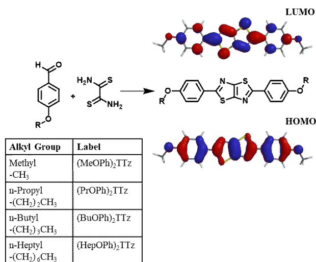
Figure 1. Schematic for the synthesis of Dialkoxyphenyl thiazolo[5,4- d ]thiazole is shown above along with electrostatic potential maps of ground state (HOMO) and first singlet excited state (LUMO) emphasizing the D-A-D character.
