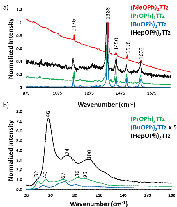
Figure 7. Micro-Raman Spectra of TTz crystals.
