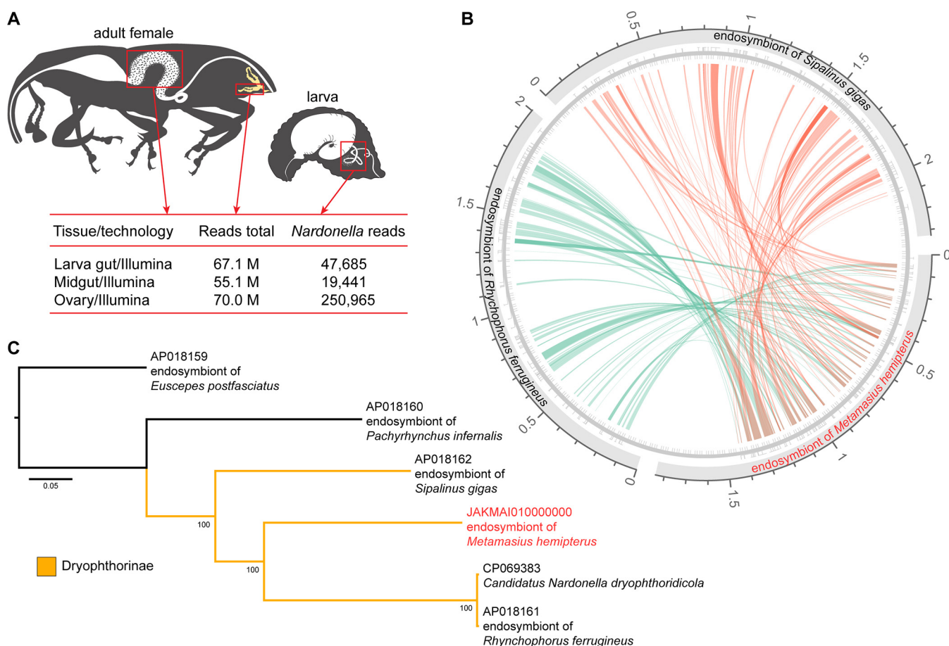
FIG 1 “ Candidatus Nardonella dryophthoridicola ” strain NARMHE1 draft genome assembly. (A) Determination of the most suitable tissue for recovering symbiont sequences. (B) Synteny circus plot showing rearrangement of some relevant genes on resulting draft genome compared with other Dryophthorinae endosymbiont Nardonella genomes. (C) Maximum-likelihood tree constructed on RAxML with all available Nardonella genomes. GenBank accession numbers of the sequences used are AP018159, endosymbiont of Euscepes postfasciatus ; AP018160, endosymbiont of Pachyrhynchus infernalis ; AP018161, endosymbiont of Rhynchophorus ferrugineus ; AP018162, endosymbiont of Sipalinus gigas ; CP069383, “ Candidatus Nardonella dryophthoridicola ”; and JAKMAI010000000, endosymbiont of Metamasius hemipterus (this study).
