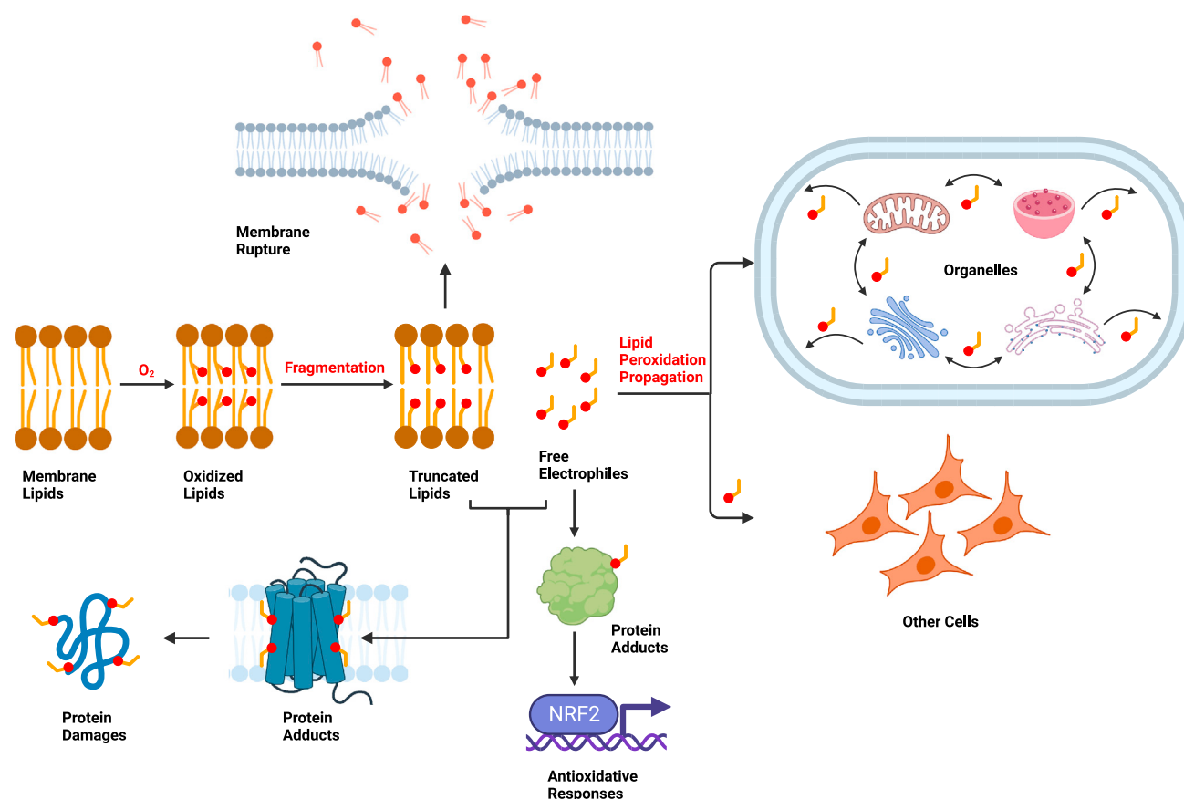
Figure 5. Proposed roles of truncated lipids and lipid electrophiles derived from lipid peroxidation in ferroptosis
