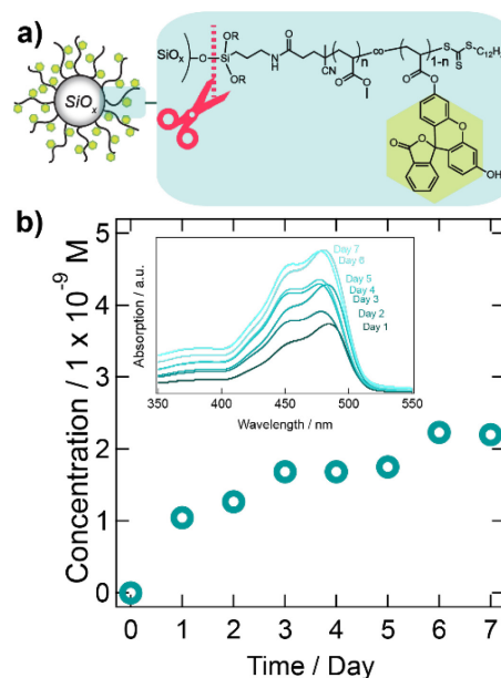
Figure 2. (a) Cartoon schematic of the fluorescein photocatalytic polymer brush glass beads ( \text{FPB@SiO}_x , not drawn to scale) and the hydrolytic -\text{Si}-\text{O}- bond highlighted. (b) UV/vis spectroscopy depicts the increasing appearance of fluorescein (photocatalyst) characteristic absorption in water, suggesting hydrolysis and leaching into the solution.
