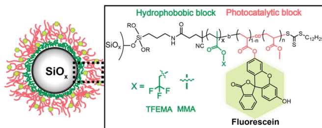
Figure 1. The chemical structure of incorporating a hydrophobic protective shell (PTFEMA or PMMA) diblock copolymer brush for the prevention of hydrolysis. The hydrophobic-block-photoactive polymer brush is tethered to a solid \text{SiO}_x support (micron-scale bead) and can be used for heterogeneous photocatalysis. The cartoon polymer brush functionalized bead is not drawn to scale.
