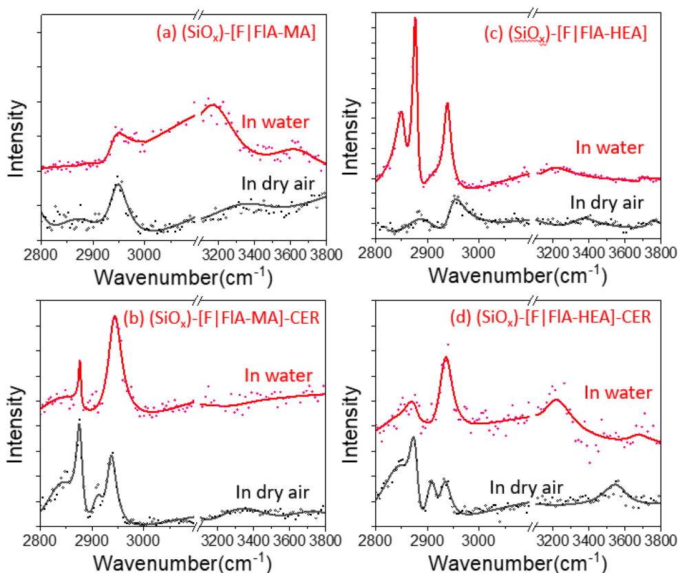
Figure 8. SFG spectra of (a) (\text{SiO}_x) -[F|FIA-MA], (b) (\text{SiO}_x) -[F|FIA-MA]-CER, (c) (\text{SiO}_x) -[F|FIA-HEA], and (d) (\text{SiO}_x) -[F|FIA-HEA]-CER brushes on flat substrates in dry air and in liquid water. The polarization combination was s- for SFG signal, s- for 532nm input beam, and p- for tunable IR beam.
