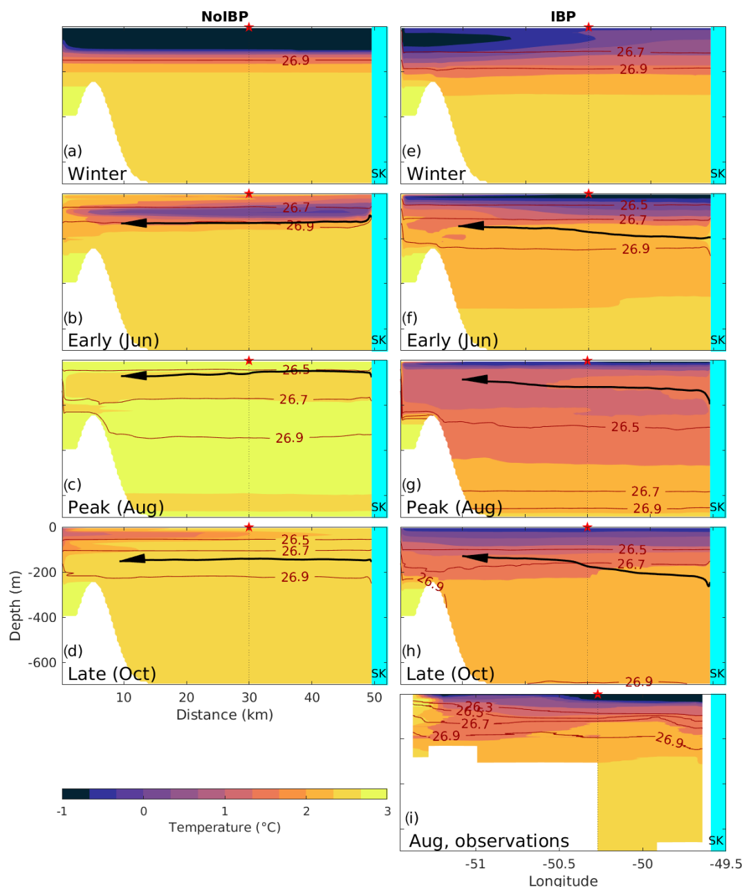
Figure 3. Along-fjord temperature sections of Ilulissat Icefjord with icebergs (e–h, IBP) and without icebergs (a–d, NoIBP), for the winter (March), early season (June), peak summer (August) and late season (October), as a snapshot along the centreline of the fjord. (i) Observed temperature section from XCTD data in August 2014 (Beaird et al., 2017), interpolated from XCTD locations marked in Fig. 1. Red contours mark the isopycnals of 26.3, 26.5, 26.7 and 26.9 \text{kg m}^{-3} . Black arrows indicate the centreline of the outflow of glacially modified water from the plume (see also Fig. 4).
