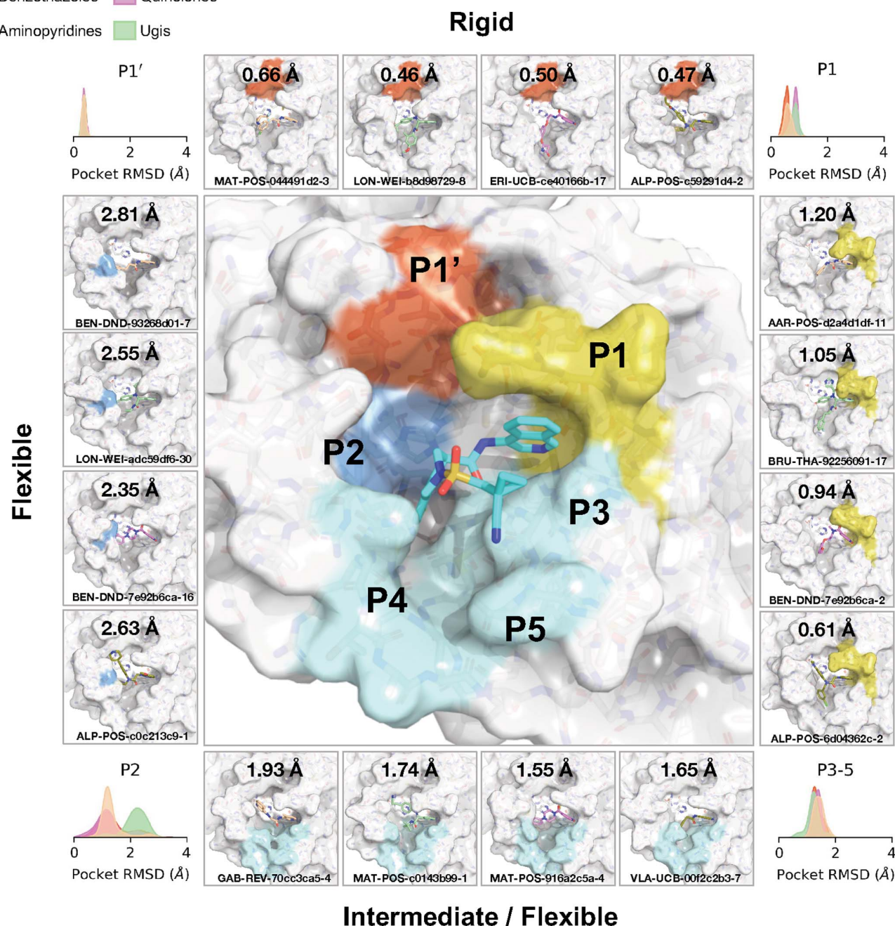
Fig. 4. Structural plasticity of the binding subpockets. The subpockets have different degrees of plasticity, which is also dependent on the chemical series (fig. S2). The corners of the figure show the distribution of sidechain root mean square deviation (RMSD) deviations from the structure of MAT-POS-e194df51-1 (middle panel; PDB: 7GAW). The boxes exemplify ligands that significantly deform the pockets.
