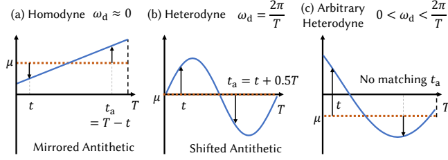
Fig. 5. Antithetic sampling for (a) homodyne, (b) heterodyne, and (c) arbitrary heterodyne mode. The ground truth integration value is \mu . In (a) and (b), we can find an antithetic pair with mirroring and shifting, respectively, that makes the primal and antithetic samples sum to \mu . But in (c), we cannot find such perfectly matching antithetic sample.
