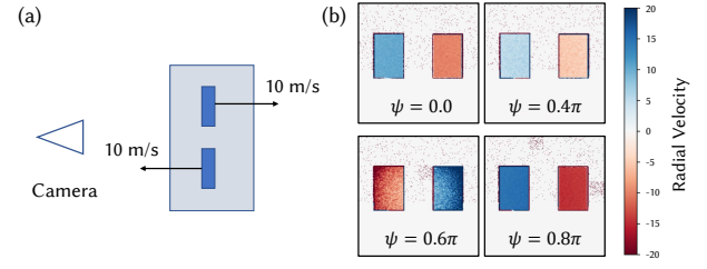
Fig. 23. We observe that for the same scene configuration shown in (a), the reconstructed radial velocity in (b) varies significantly for different phase offset \psi values. Only the left top corner ( \psi = 0 ) gives the correct velocity. We only show result of Heide et al. [2015], but similar for Hu et al. [2022].
