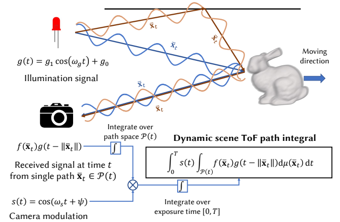
Fig. 2. Overview of ToF imaging and rendering of a dynamic scene. We show two paths \bar{x}_t that arrive at the same image pixel. In D-ToF imaging, s(t) and g(t) are high-frequency sinusoidal functions. The sinusoidal waves represent the illumination intensity at each point on the two paths.
