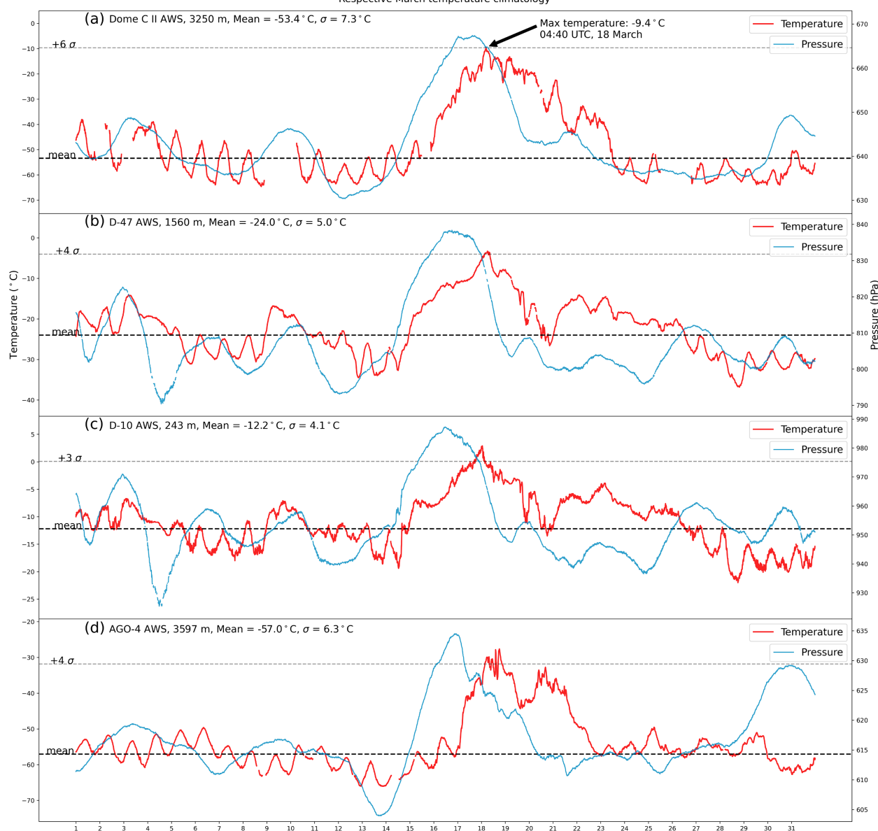
FIG. 9. March 2022 University of Wisconsin–Madison Automatic Weather Station 10-min quality-controlled temperature (red) and pressure (blue) observations and respective March temperature climatologies for (a) Dome C II, (b) D-47, (c) D-10, and (d) AGO-4. Each plot lists the AWS name, elevation, mean, and standard deviation of March 2022 temperature. The mean temperature is plotted with a thick dashed horizontal line, and the nearest integer standard deviation below the maximum temperature is plotted in a dashed horizontal line. Note the varying temperature and pressure ranges on the y axes.
