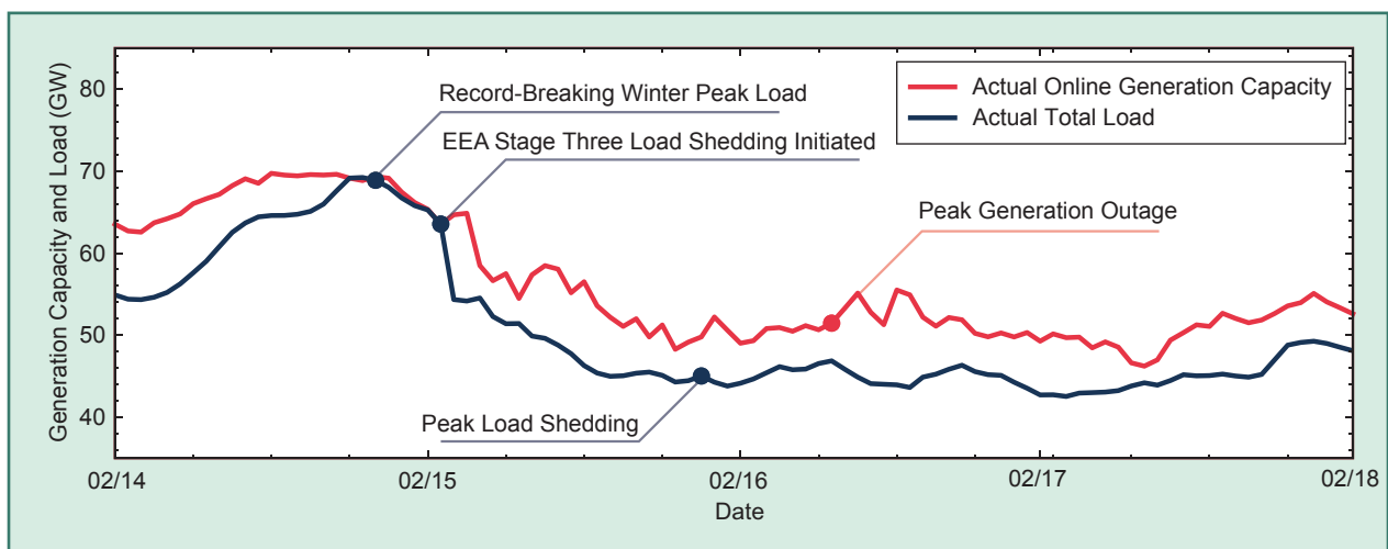
figure 5. The actual online generation capacity and load in Texas interconnection between 14–18 February 2021. EEA: Energy Emergency Alert.
