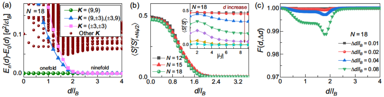
FIG. 2. (a) The low-lying energy spectra as a function of the layer distance d/l_B for the filling (\nu_1, \nu_2) = (\frac{1}{3}, -\frac{1}{3}) . Here we show only the inequivalent momentum sectors. There are ninefold degenerate states at larger d/l_B . (b) The correlator \langle S_i^y S_{i+N_\phi/2}^y \rangle versus layer distances d/l_B . The inset shows \langle S_i^y S_j^y \rangle as a function of the orbital distance |i - j| . Here, i, j = 1, \dots, N_\phi are orbital indices and the corresponding distance is |i - j|L/N_\phi . From top to bottom, d/l_B ranges from 0 to 2.4 with interval 0.4. (c) The fidelity F(d, \Delta d) as a function of the layer distances d/l_B taking different intervals of parameters \Delta d/l_B . Note that with decreased \Delta d the dip is weakened.
