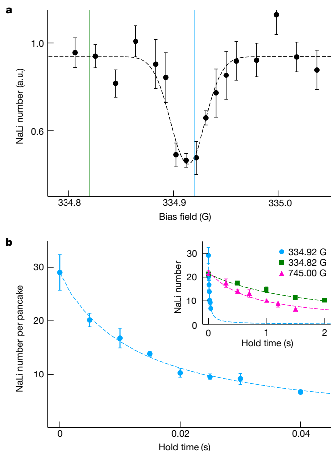
Fig. 1 | Resonant molecular loss. a , The remaining molecule number after holding for 30\text{ ms} at a target field is mapped out for various magnetic fields near 334.9\text{ G} . Molecule numbers are normalized by the number without the hold. Each data point represents three to six measurements with and without 30\text{-ms} hold and the error bars are one standard deviation. The dashed black line is a Gaussian fit. The vertical blue (green) line indicates the field in which the molecular decay curve in blue (green) is obtained in b . b , The main plot shows the decay curve near the centre of the resonance ( 334.92\text{ G} ) within 50\text{ ms} . The inset shows decay curves away from the resonance at 334.82\text{ G} (green squares), at 745.00\text{ G} (red triangles) and at 334.92\text{ G} (blue circles) over 2\text{ s} . Dashed lines are fits to a simple model for two-body loss using mean square regression (see Methods for details). Data values represent the average and error bars represent one standard deviation of the mean, estimated from statistical errors of three to six measurements.
