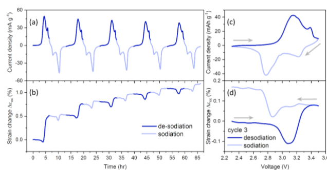
Figure 2. (a) Current density and (b) strain change in \text{NaCrO}_2 cathodes with respect to time during the cyclic voltammetry at 50 \mu\text{V/s} rate between 2.3 to 3.5 V. (c) current density and (d) strain change with respect to voltage during 3 rd cycle, the strain is set to zero at the beginning of the 3 rd cycle.
