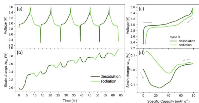
Figure 3: (a) Voltage profile and (b) strain evolution of \text{NaCrO}_2 cathode versus time during cycling at C/25 between 2.3 V - 3.6 V for five cycles. (c) Voltage and (d) strain change is plotted against specific capacity in the third cycle and strain was set to zero at the beginning of third cycle for better comparison.
