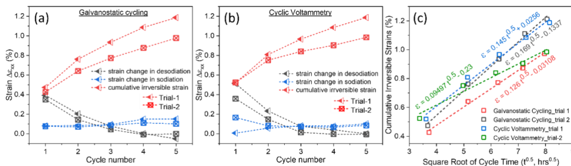
Figure 5. Strain trends during desodiation, sodiation process and irreversible strain generation during (a) galvanostatic cycling and (b) cyclic voltammetry in each cycle; (c) cumulative irreversible strain evolution in \text{NaCrO}_2 electrode plotted against the square root of cycle time. The original data is from Figures 2 and 3 and Supp Figures S8-9. Trails 1 and 2 show the repeated experimental results performed under the same galvanostatic cycling and cyclic voltammetry for Figure a and b, respectively.
