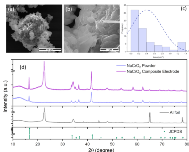
Figure 1. (a, b) SEM images of pristine \text{NaCrO}_2 powder, (c) particle size distribution of \text{NaCrO}_2 powder and (d) X-ray diffraction pattern of pristine \text{NaCrO}_2 , a composite electrode of \text{NaCrO}_2 , aluminium foil (utilized as a current collector for composite electrode) and the JCPDS file of \text{NaCrO}_2 for reference.
