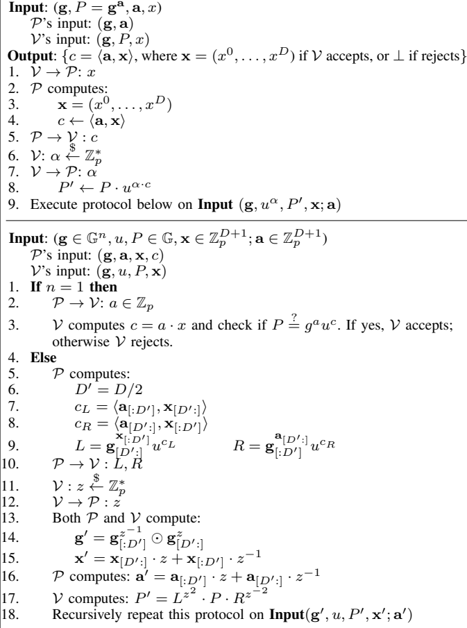
Fig. 5: IPA-based Verifiable Polynomial Evaluation.
