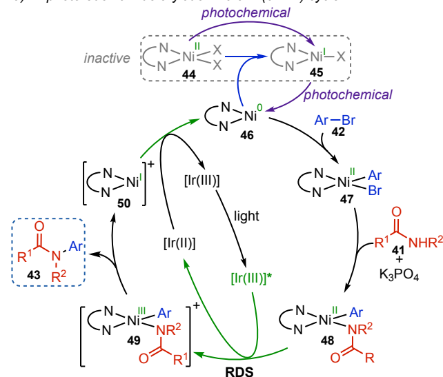
Figure 7. A Ni(0/II/III) cycle facilitates Ni-photoredox amide arylations
