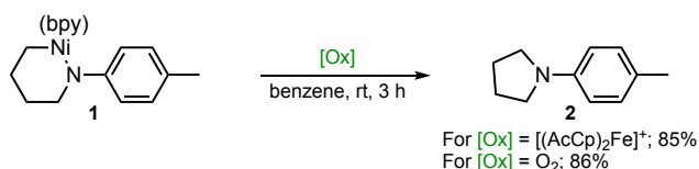
Scheme 1. Seminal stoichiometric and catalytic examples of accelerating C–N reductive elimination from Ni(III) complexes
