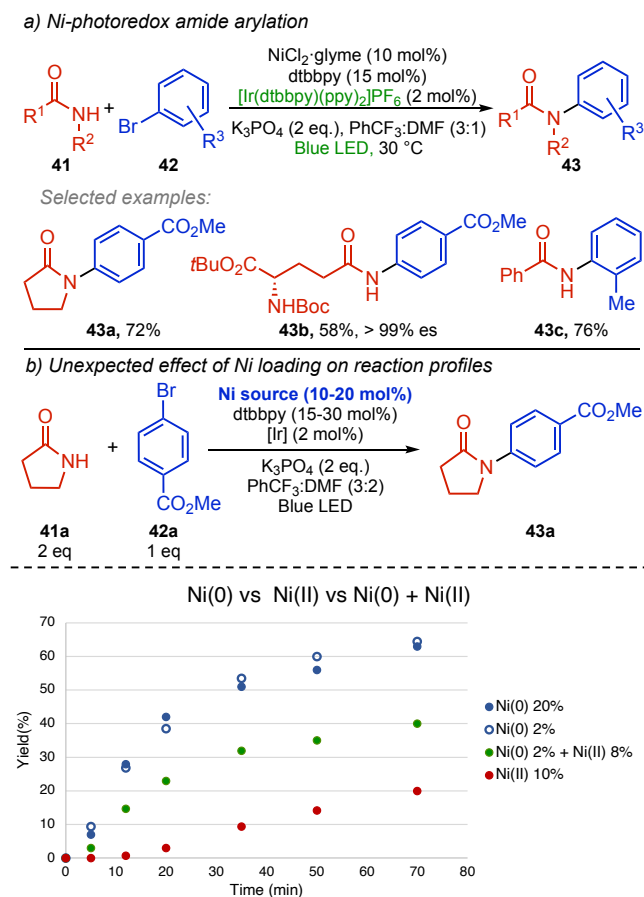
Figure 6. Ni-photoredox amide arylations scope and Ni(II) loading effects
