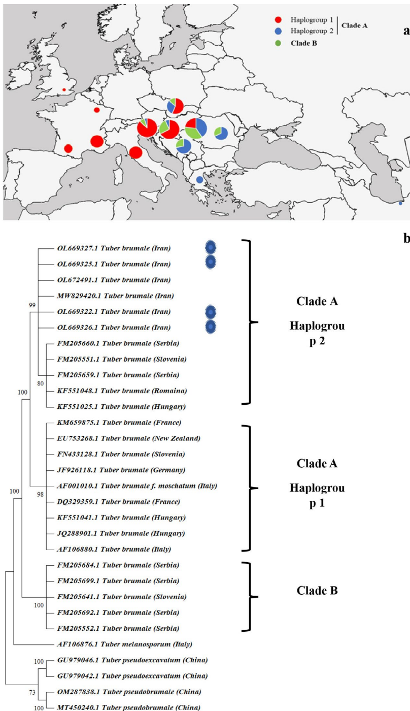
Fig. 2. The distribution and phylogenetic relationship of Tuber brumale populations: a) The distribution and habitat of T. brumale according to the report made by MERÉNYI et al. (2014) in addition to our sampling location in Iran (blue dot); b) The phylogenetic relationship between Iranian T. brumale (blue asterisk) and populations in Eurasia.
