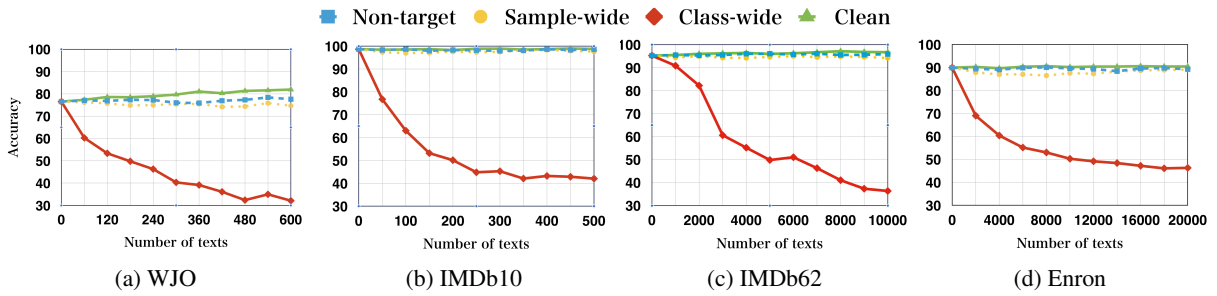
Figure 6: Experiment results on incremental warm-start poisoning
