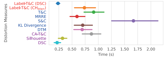
Fig. 5. Results of the scalability analysis. Name and line colors match with Fig. 4. Label-T&C [DSC] (dark blue) is on par with CVMs (Silhouette, DSC), while Label-T&C [ CH_{brwn} ] is similar to most of the other measures. S&C is the slowest.
