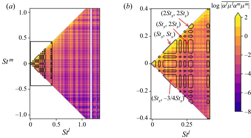
Figure 9. (a) The principle region of bispectrum for all modes containing 99 % of cumulative TKE and sparse-selected modes. (b) Zoomed-in view.
