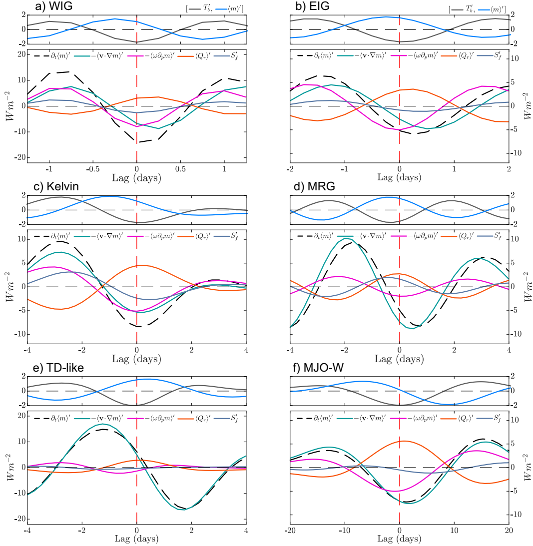
FIG. 7. The larger bottom plot for each panel shows the area-average anomaly terms of the column MSE budget of Eq. (5): \partial_t \langle m \rangle' (dashed black), -\langle \mathbf{v} \cdot \nabla m \rangle' (green), -\langle \omega \partial_p m \rangle' (magenta), \langle Q_r \rangle' (dark orange), and S_f' (light blue). The smaller top plot for each panel shows the evolution of the T_b (gray) and column MSE (light blue). Lag regression of budget terms are based on PC1 time series (normalized) of the corresponding CCWs averaged over 10°S–10°N, 80°–20°W for WIG, EIG, Kelvin, and MJO-W waves; 0°–15°N, 120°–70°W for MRGs; and 0°–15°N, 60°–0°W for TD-like wave. Anomalies are scaled to one standard deviation PC perturbation of the corresponding CCWs.
