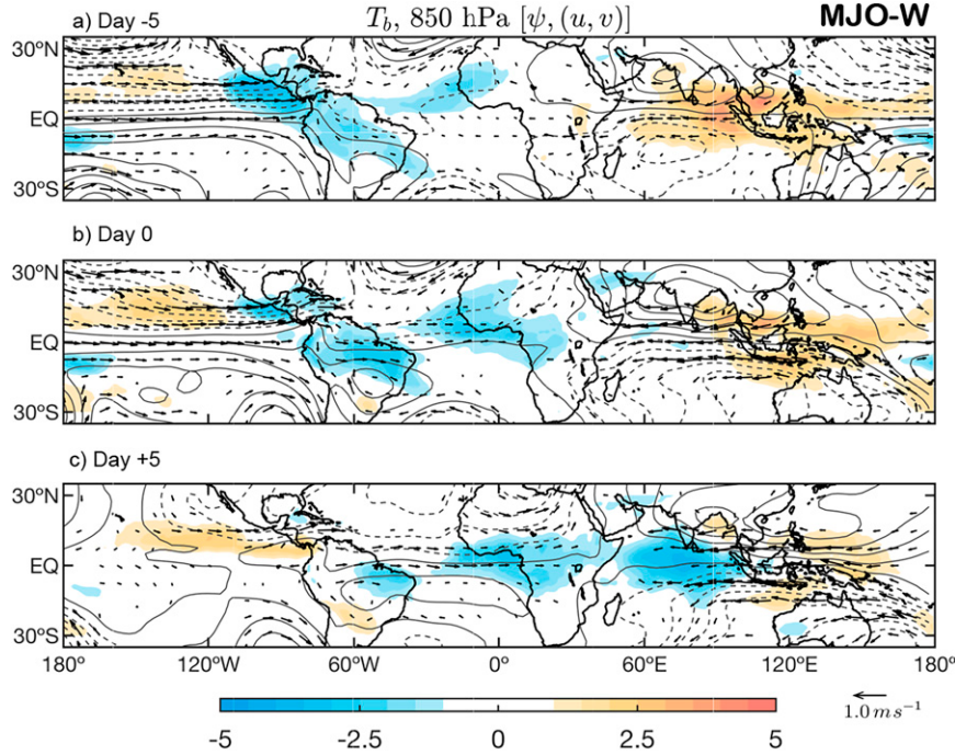
FIG. 5. As in Fig. 2, but for the MJO-W wave for (a) day -5 , (b) day 0 , and (c) day +5 . Contours are streamfunction, and the contour interval is 2.0 \times 10^6 \text{ m}^2 \text{ s}^{-1} , with negative contours dashed.
