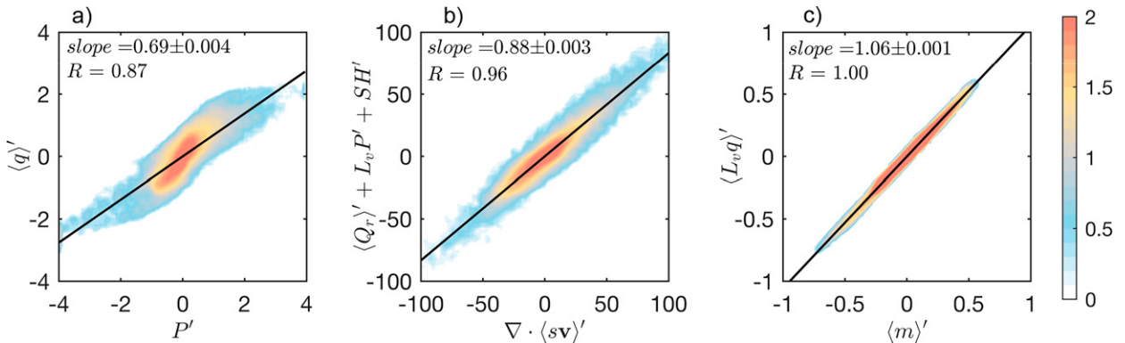
FIG. 6. Scatterplots of (a) P' vs \langle q \rangle' , (b) \nabla \cdot \langle s \mathbf{v} \rangle' vs \langle Q_r \rangle' + L_v P' + SH' , and (c) \langle m \rangle' vs \langle L_v q \rangle' for the TD-like waves. The shading represents the base-10 logarithm of the number of points within 0.1 \text{ mm} \times 0.1 \text{ mm} bins in (a), 2 \text{ W m}^{-2} \times 2 \text{ W m}^{-2} bins in (b), and 2.5 \times 10^5 \text{ J m}^{-2} \times 2.5 \times 10^5 \text{ J m}^{-2} bins in (c). Anomalies are obtained by regressing all fields against the PC1 (normalized, TD-like) over the 0^\circ – 15^\circ\text{N} , 60^\circ – 0^\circ\text{W} domain. The linear fit obtained from linear least squares fit is shown as a solid black line. The slope of the linear fit and the correlation coefficient are shown in the top-left of each panel.
