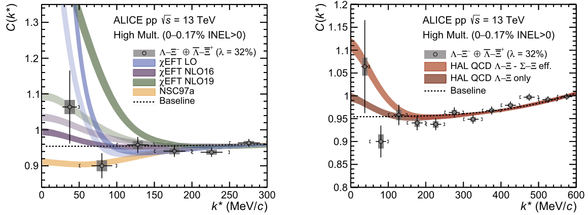
Fig. 2. Experimental \Lambda - \Xi correlation function with statistical (vertical black lines) and systematic (gray boxes) uncertainties. The square brackets show the bin width of the measurement and the horizontal black lines represent the statistical uncertainty in the determination of the mean k^* for each bin. Left panel: Comparison to LO [11] and NLO [16] \chi EFT and NSC97a [12] potentials evaluated with the Lednický-Lyuboshits model [40,41]. In the \chi EFT models the darker and light bands correspond to the version with the lower and higher cut-off value, respectively. Right panel: Comparison with Lattice QCD calculations by the HAL QCD Collaboration [2] using an effective potential including the coupling to \Sigma - \Xi (orange) and the \Lambda - \Xi elastic potential alone (red). The width of the bands in both panels correspond to the systematic uncertainties of the fit as described in the text. The dotted black line represents the result of the baseline fit assuming no \Lambda - \Xi strong interaction.
