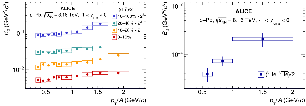
Fig. 2. Coalescence parameters B_2 (left panel) and B_3 (right panel) as a function of p_T/A , measured for deuterons and ^3\text{He} , respectively. Statistical uncertainties are represented as vertical lines whereas boxes represent the systematic ones.
