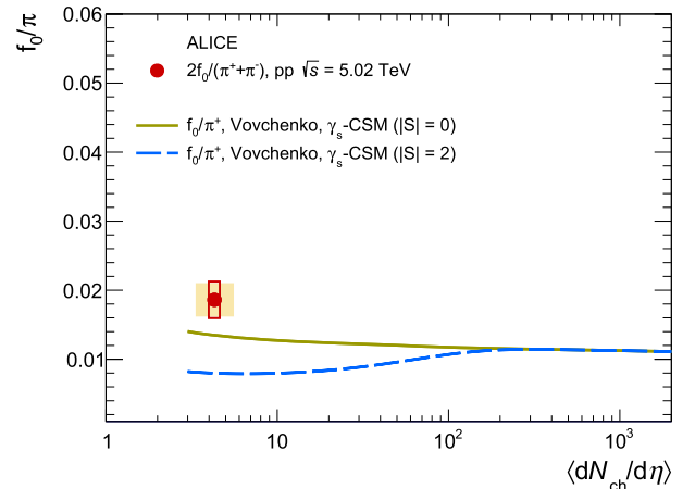
Fig. 5. The 2f_0/(\pi^+ + \pi^-) ratio measured in pp collisions at \sqrt{s} = 5.02 TeV [61] is compared to two distinct predictions for f_0/\pi^+ from a canonical statistical model ( \gamma_s - \text{CSM} [68], see text for details) as a function of \langle dN_{ch}/d\eta \rangle . The two calculations differ by the assumed strangeness content of f_0(980) and correspond to zero total strangeness, |S| = 0 and |S| = 2 . The height of the hollow red box represents the total uncertainty on the ratio, its width represents the uncertainty on the \langle dN_{ch}/d\eta \rangle . The relative uncertainty of 13% due to the branching ratio correction [42] is shown as a yellow box with an arbitrary horizontal width for visibility.
