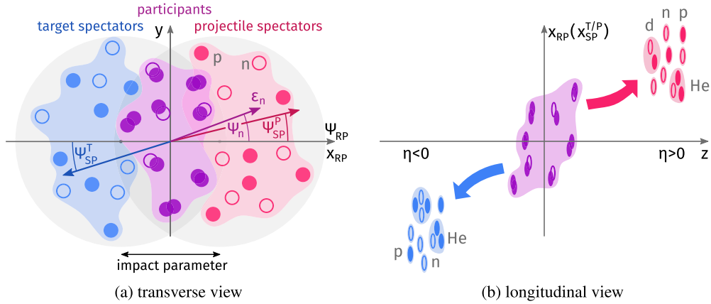
Fig. 1. A sketch of the geometry of a non-central heavy-ion collision in the (a) transverse ( x_{RP} , y ) and (b) reaction ( x_{RP} , z ) planes. The x_{RP} axis points along the direction of the impact parameter given by the distance between the centers of the colliding nuclei, while the z axis is oriented along the direction of the colliding nuclei. The full (open) circles represent the protons (neutrons) from projectile (red) and target (blue) nuclei. The participant nucleons are shown in purple. In panel (a), the arrows indicate the eccentricity vectors ( \epsilon_n is shown as example) and corresponding reaction ( \Psi_{RP} ), projectile/target spectator ( \Psi_{SP}^{P,T} ), and participant (multiple \Psi_n , n \geq 1 ) plane angles. Panel (b) shows the outward deflection, indicated by curved arrows, of the spectators and fragmentation products of the projectile ( \eta > 0 ) and target ( \eta < 0 ) recoil nuclei, such as protons ( p ), neutrons ( n ), and nuclei (deuteron, helium, etc).
