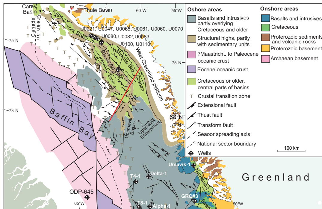
Figure F2. Tectonic elements map of northeast Baffin Bay showing position of Expedition 400 seismic transect (red line) (see Figure F4) and existing deep drilling sites (IODP, IODP, and exploration wells). Adapted from Gregersen et al. (2022).
