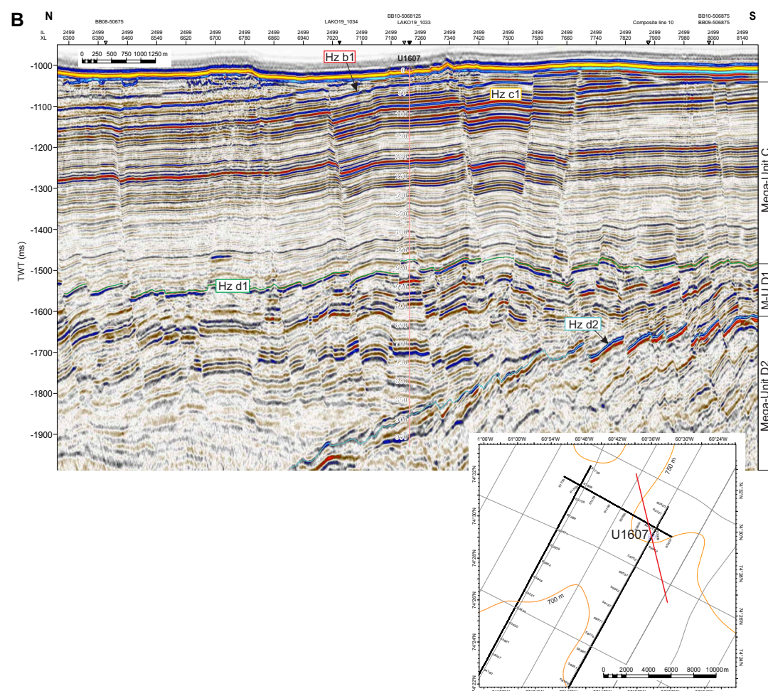
Figure F14 (continued).
