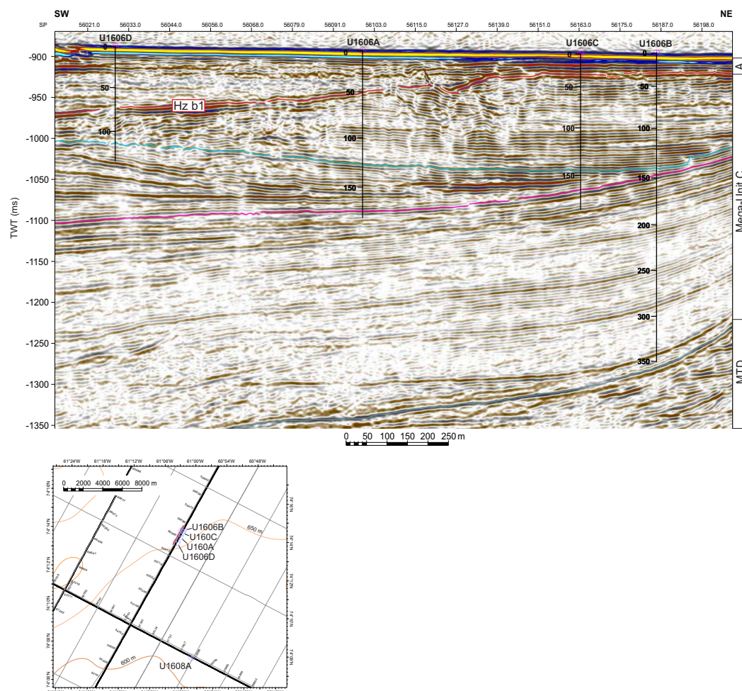
Figure F12. Top: seismic profile (LAKO19_1033) showing location of Site U1606 on outer shelf of Melville Bugt, northwest Greenland. Vertical scale on hole lines are meter depth based on preferred time-depth model. SP = shotpoint, TWT = two-way travelttime, MTD = mass transport deposit. Bottom: close-up bathymetry map with seismic survey lines in vicinity of Site U1606. Gray line grid = regional 2-D seismic data (TGS), black line grid = high-resolution multichannel seismic data (LAKO19).
