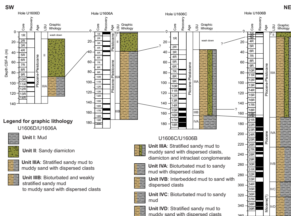
Figure F13. Lithostratigraphic summary, Site U1606.
